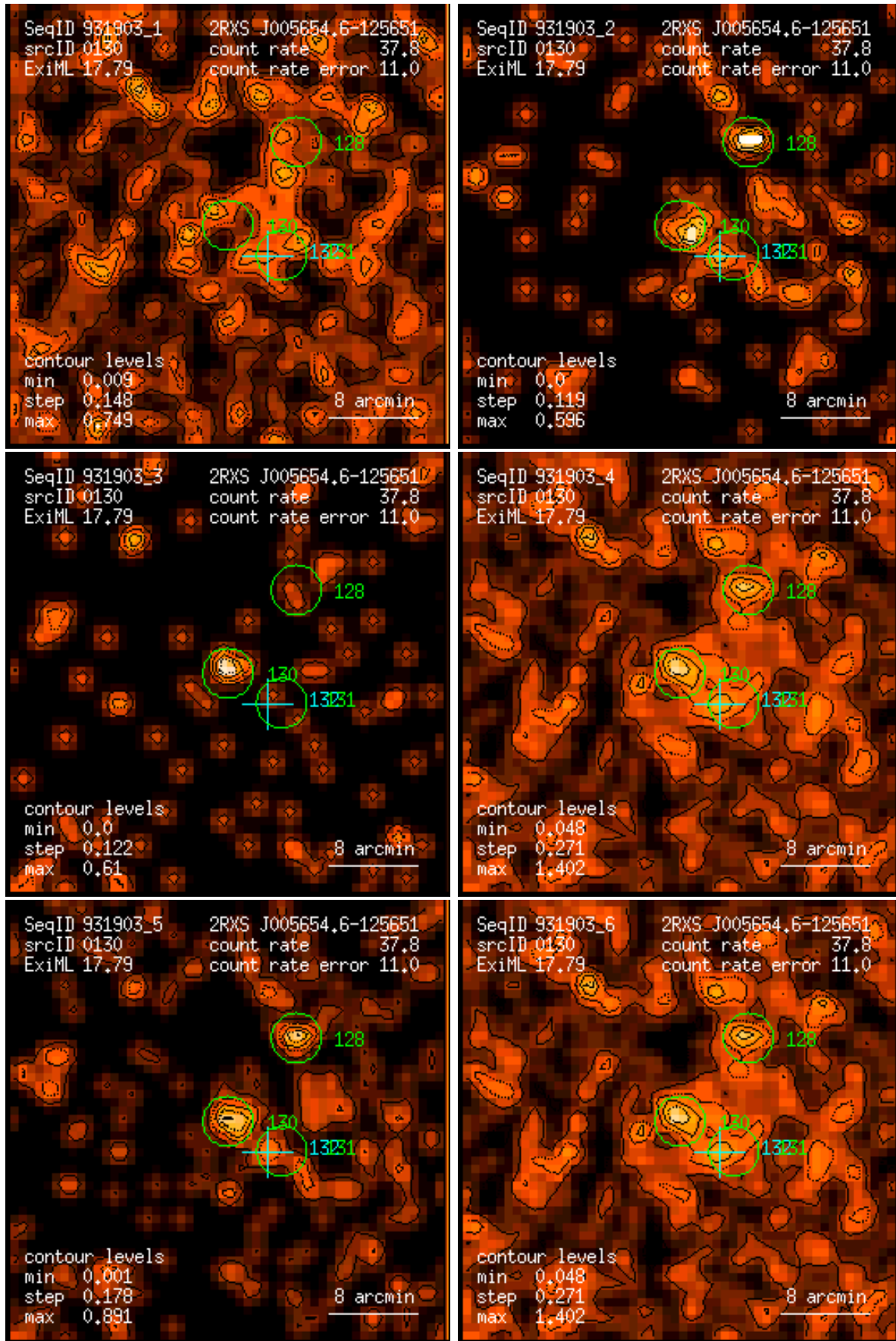
Figure 130: RASS 931903: detection 0130: band rate images, Gaussian filter: (1) PSPC channels 11 – 41, (2) 52 – 90, (3) 91 – 201, (4) 11 – 235, (5) 52 – 201, (6) 11 – 201. Broad band rates in counts/ks. Band rate contour levels in counts/ks/arcmin 2 .
