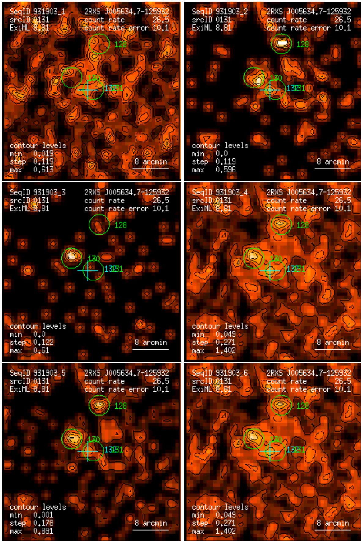
Figure 131: RASS 931903: detection 0131: band rate images, Gaussian filter: (1) PSPC channels 11 – 41, (2) 52 – 90, (3) 91 – 201, (4) 11 – 235, (5) 52 – 201, (6) 11 – 201. Broad band rates in counts/ks. Band rate contour levels in counts/ks/arcmin 2 .
