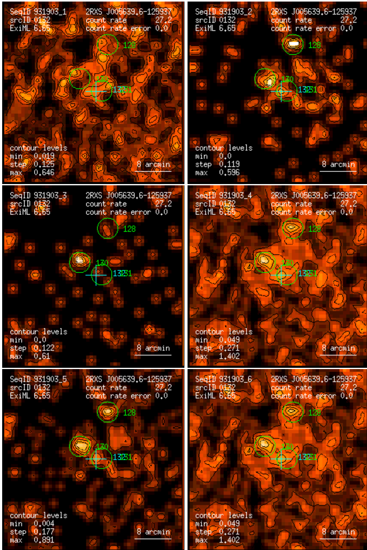
Figure 132: RASS 931903: detection 0132: band rate images, Gaussian filter: (1) PSPC channels 11 – 41, (2) 52 – 90, (3) 91 – 201, (4) 11 – 235, (5) 52 – 201, (6) 11 – 201. Broad band rates in counts/ks. Band rate contour levels in counts/ks/arcmin 2 .
