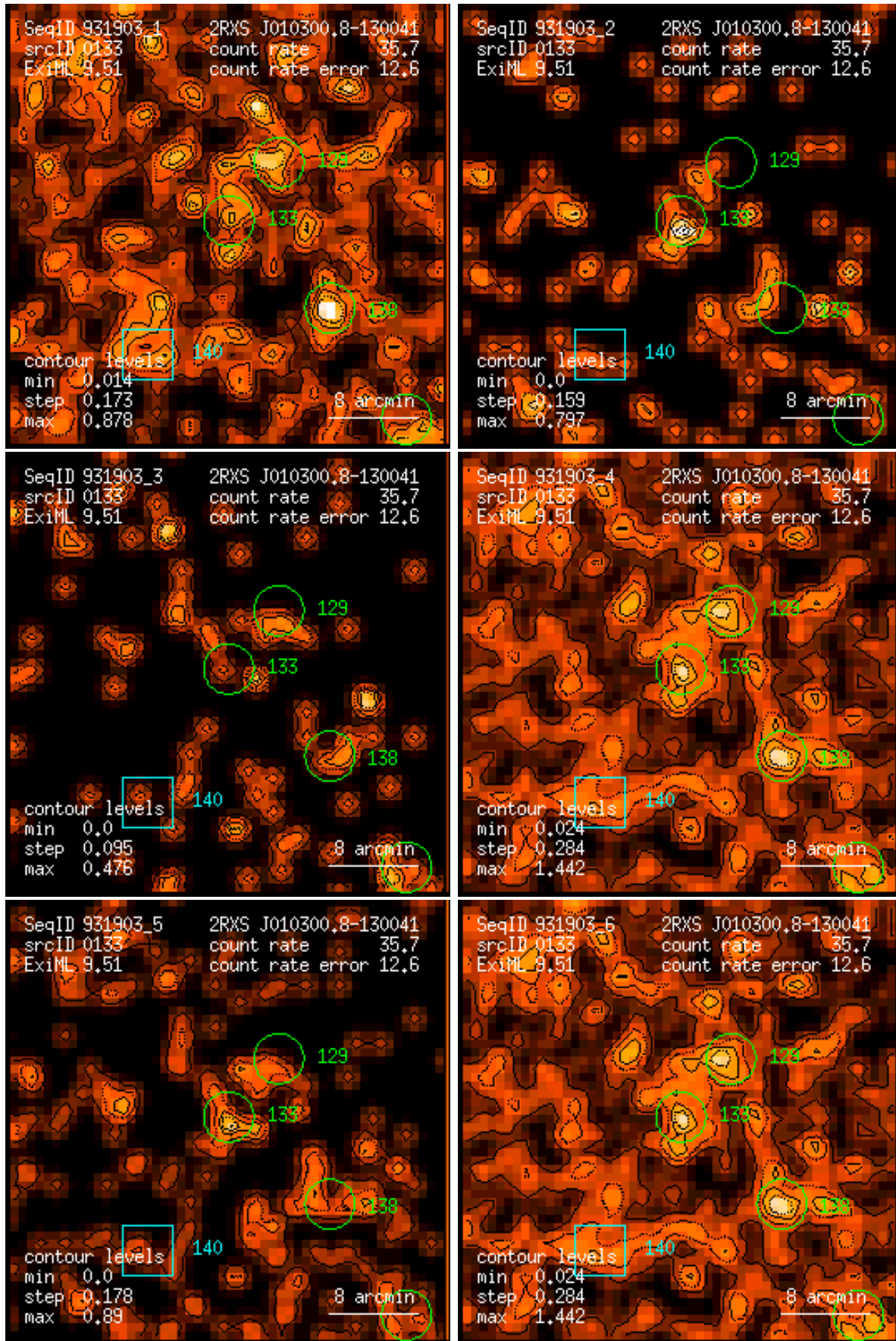
Figure 133: RASS 931903: detection 0133: band rate images, Gaussian filter: (1) PSPC channels 11 – 41, (2) 52 – 90, (3) 91 – 201, (4) 11 – 235, (5) 52 – 201, (6) 11 – 201. Broad band rates in counts/ks. Band rate contour levels in counts/ks/arcmin 2 .
