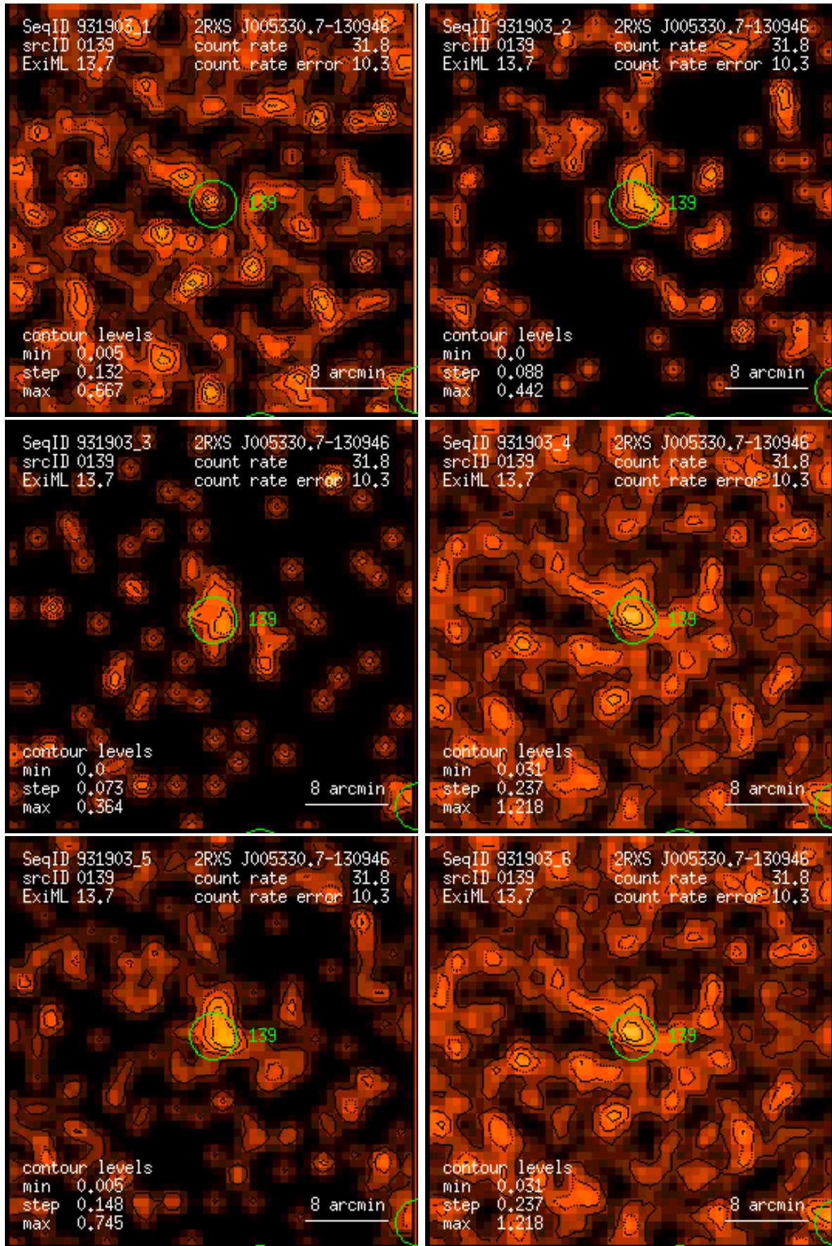
Figure 139: RASS 931903: detection 0139: band rate images, Gaussian filter: (1) PSPC channels 11 – 41, (2) 52 – 90, (3) 91 – 201, (4) 11 – 235, (5) 52 – 201, (6) 11 – 201. Broad band rates in counts/ks. Band rate contour levels in counts/ks/arcmin 2 .
