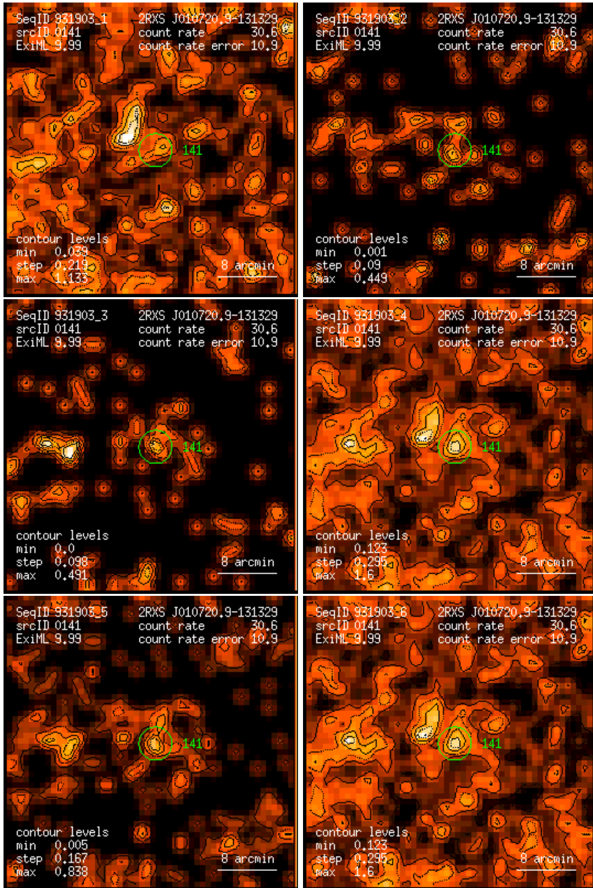
Figure 141: RASS 931903: detection 0141: band rate images, Gaussian filter: (1) PSPC channels 11 – 41, (2) 52 – 90, (3) 91 – 201, (4) 11 – 235, (5) 52 – 201, (6) 11 – 201. Broad band rates in counts/ks. Band rate contour levels in counts/ks/arcmin 2 .
