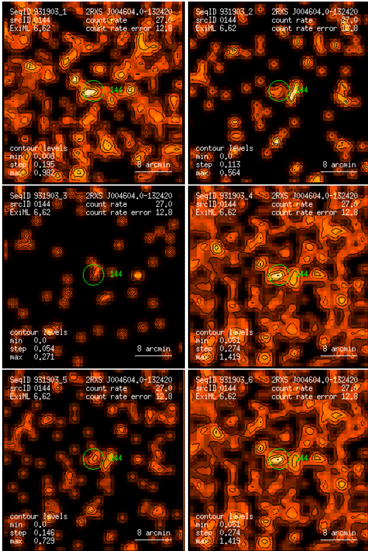
Figure 144: RASS 931903: detection 0144: band rate images, Gaussian filter: (1) PSPC channels 11 – 41, (2) 52 – 90, (3) 91 – 201, (4) 11 – 235, (5) 52 – 201, (6) 11 – 201. Broad band rates in counts/ks. Band rate contour levels in counts/ks/arcmin 2 .
