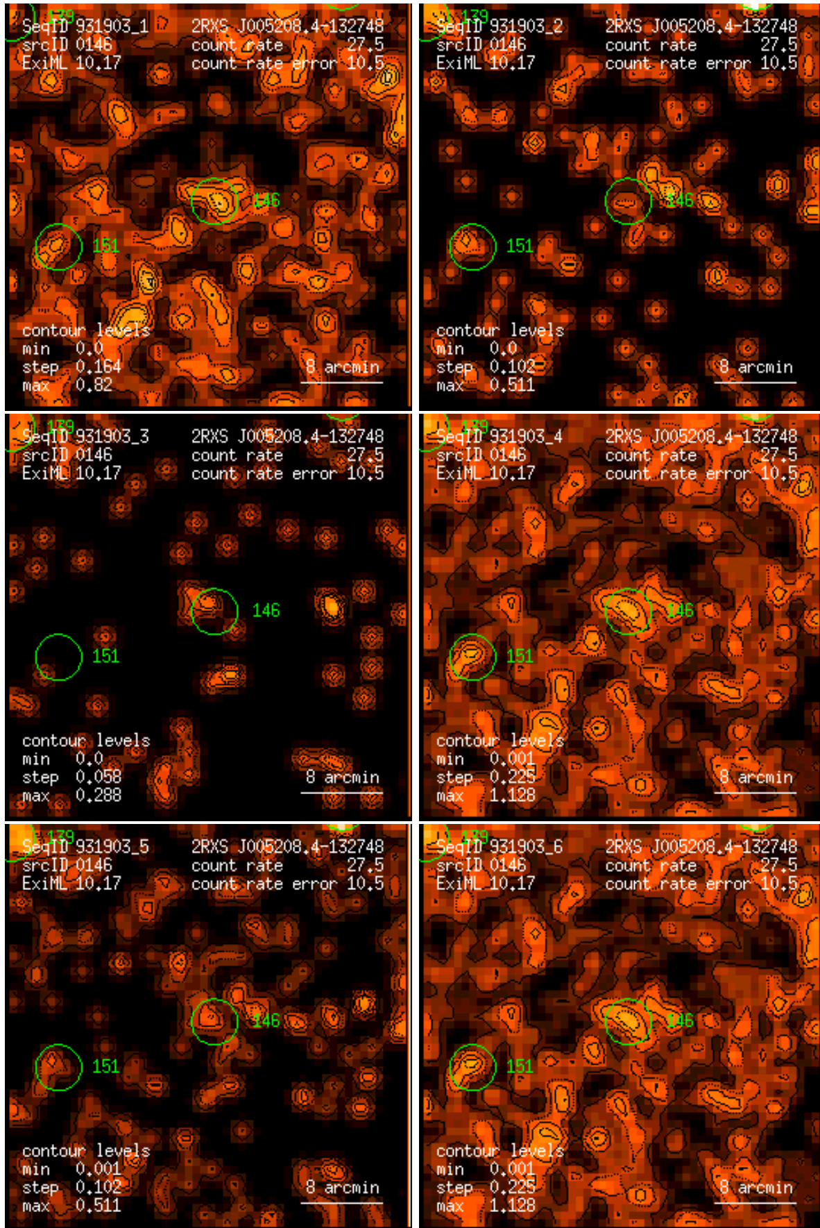
Figure 146: RASS 931903: detection 0146: band rate images, Gaussian filter: (1) PSPC channels 11 – 41, (2) 52 – 90, (3) 91 – 201, (4) 11 – 235, (5) 52 – 201, (6) 11 – 201. Broad band rates in counts/ks. Band rate contour levels in counts/ks/arcmin 2 .
