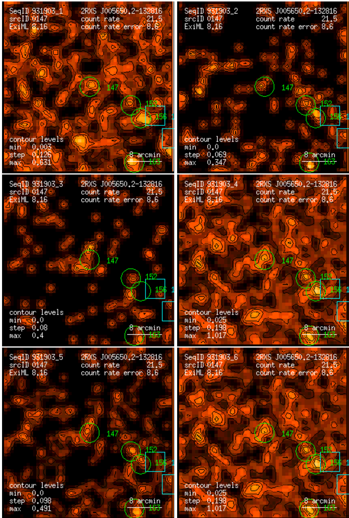
Figure 147: RASS 931903: detection 0147: band rate images, Gaussian filter: (1) PSPC channels 11 – 41, (2) 52 – 90, (3) 91 – 201, (4) 11 – 235, (5) 52 – 201, (6) 11 – 201. Broad band rates in counts/ks. Band rate contour levels in counts/ks/arcmin 2 .
