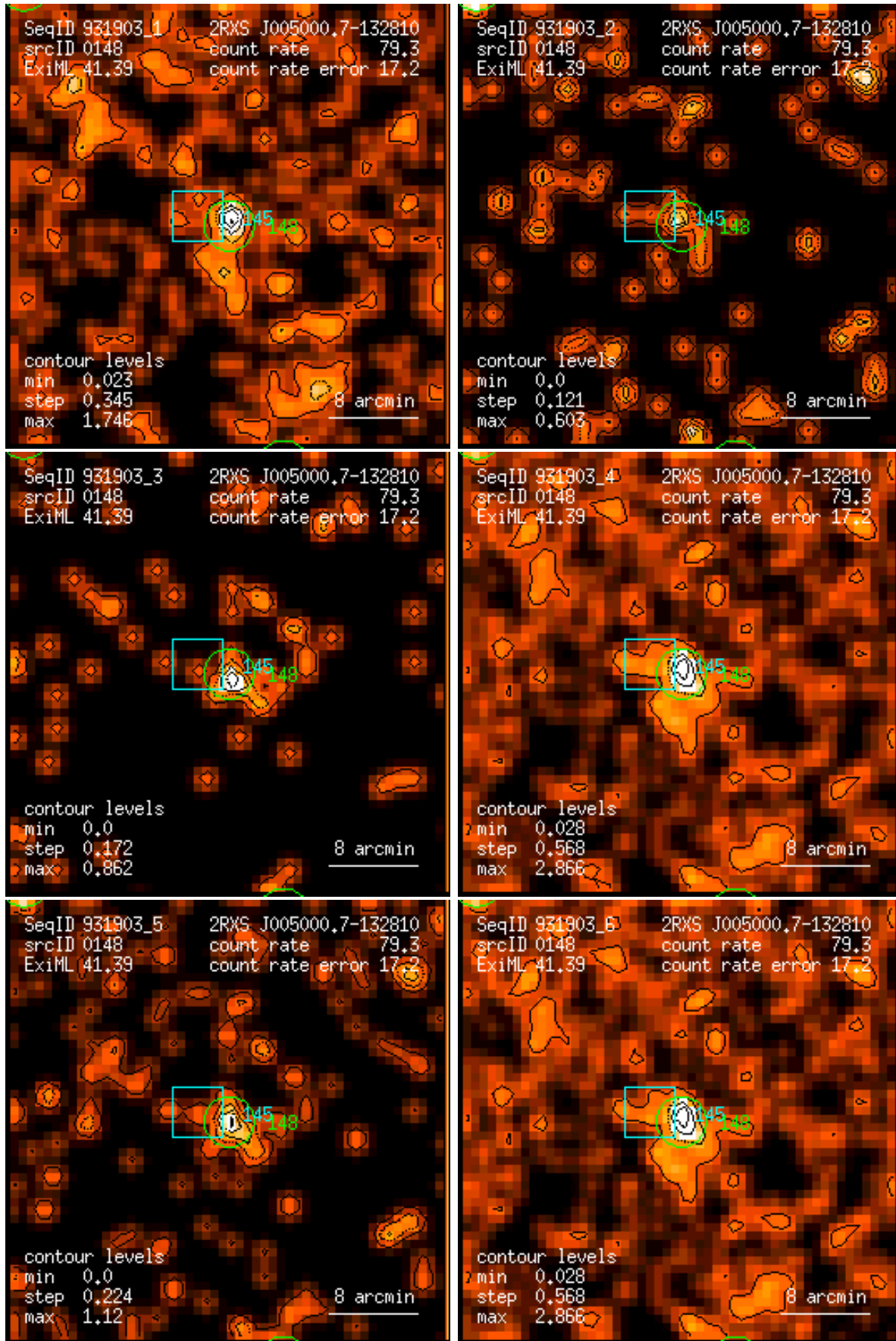
Figure 148: RASS 931903: detection 0148: band rate images, Gaussian filter: (1) PSPC channels 11 – 41, (2) 52 – 90, (3) 91 – 201, (4) 11 – 235, (5) 52 – 201, (6) 11 – 201. Broad band rates in counts/ks. Band rate contour levels in counts/ks/arcmin 2 .
