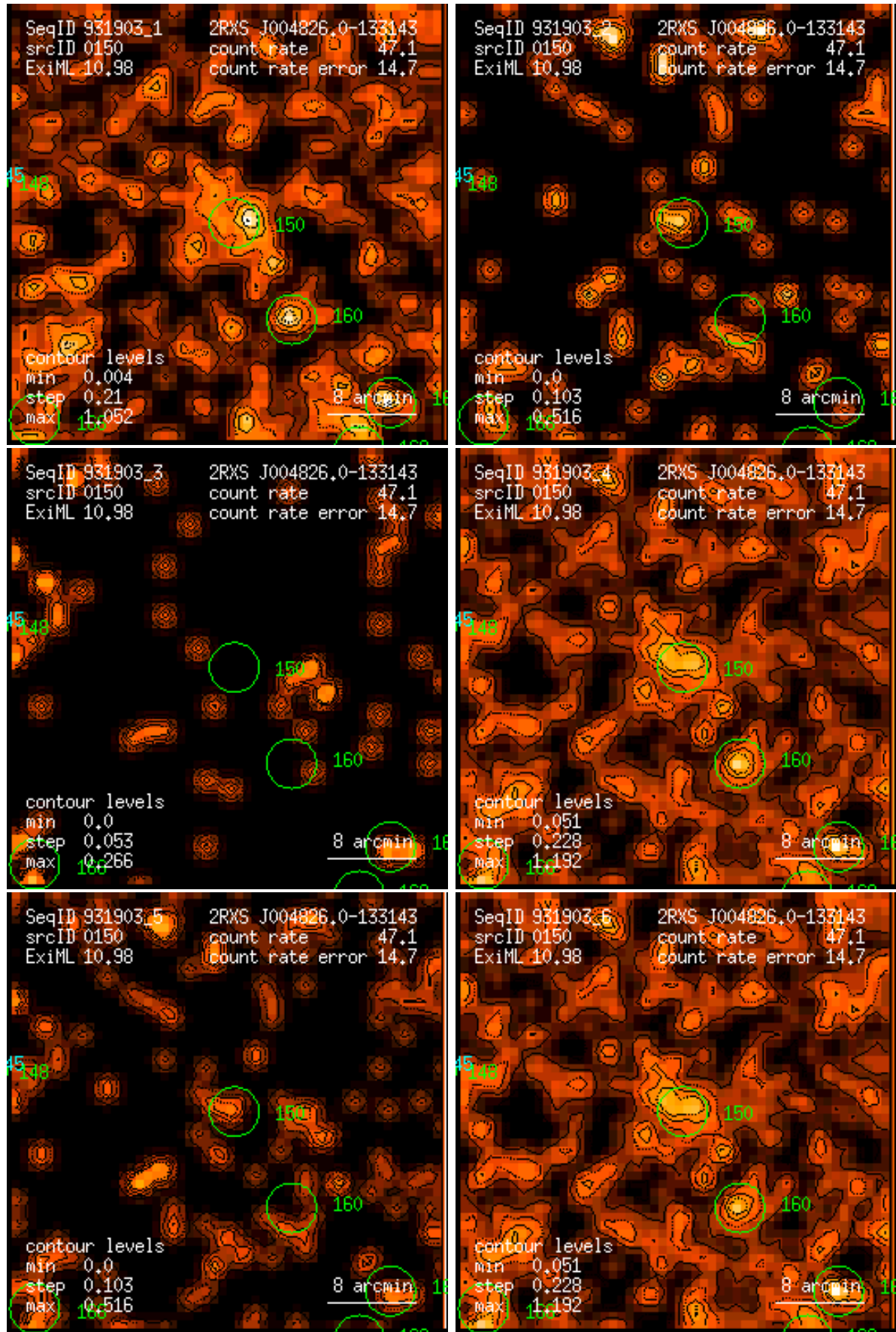
Figure 150: RASS 931903: detection 0150: band rate images, Gaussian filter: (1) PSPC channels 11 – 41, (2) 52 – 90, (3) 91 – 201, (4) 11 – 235, (5) 52 – 201, (6) 11 – 201. Broad band rates in counts/ks. Band rate contour levels in counts/ks/arcmin 2 .
