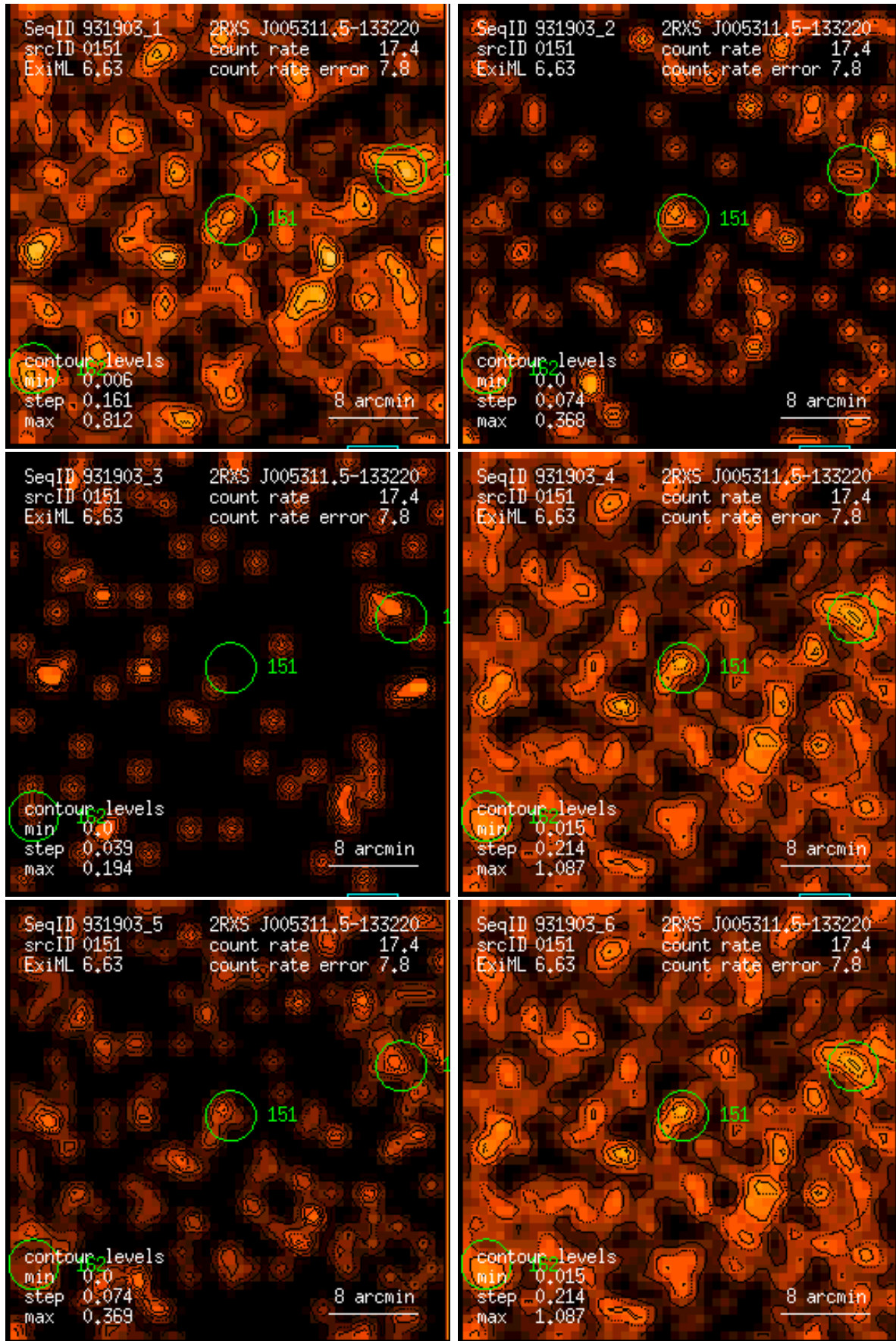
Figure 151: RASS 931903: detection 0151: band rate images, Gaussian filter: (1) PSPC channels 11 – 41, (2) 52 – 90, (3) 91 – 201, (4) 11 – 235, (5) 52 – 201, (6) 11 – 201. Broad band rates in counts/ks. Band rate contour levels in counts/ks/arcmin 2 .
