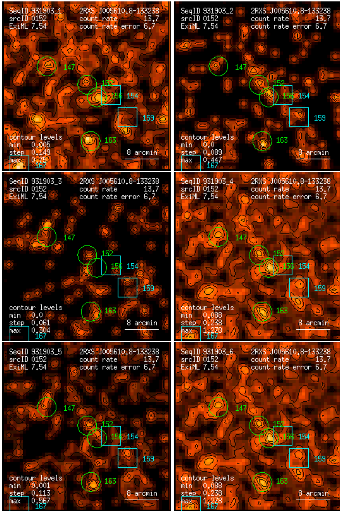
Figure 152: RASS 931903: detection 0152: band rate images, Gaussian filter: (1) PSPC channels 11 – 41, (2) 52 – 90, (3) 91 – 201, (4) 11 – 235, (5) 52 – 201, (6) 11 – 201. Broad band rates in counts/ks. Band rate contour levels in counts/ks/arcmin 2 .
