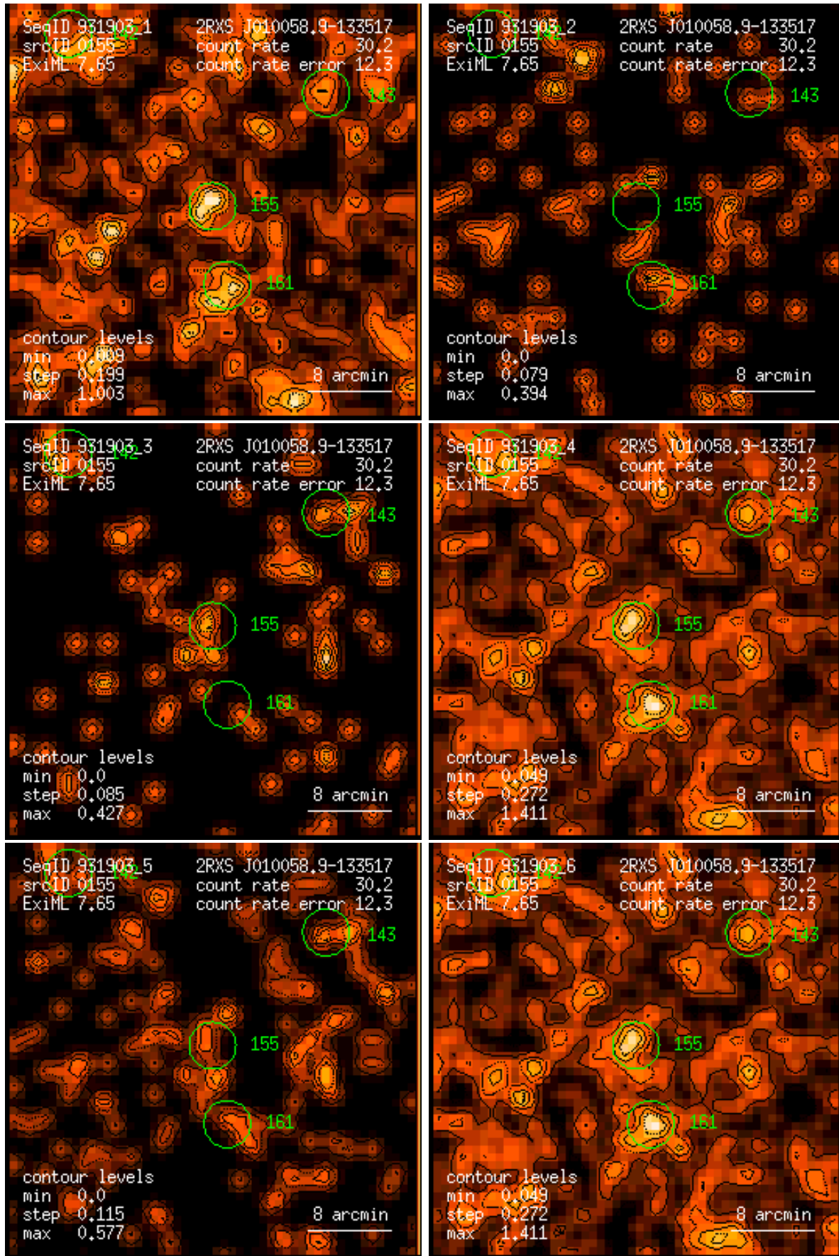
Figure 155: RASS 931903: detection 0155: band rate images, Gaussian filter: (1) PSPC channels 11 – 41, (2) 52 – 90, (3) 91 – 201, (4) 11 – 235, (5) 52 – 201, (6) 11 – 201. Broad band rates in counts/ks. Band rate contour levels in counts/ks/arcmin 2 .
