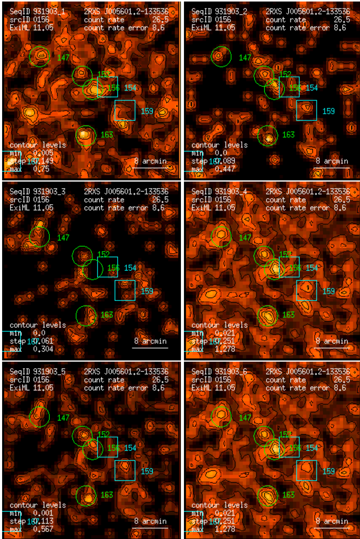
Figure 156: RASS 931903: detection 0156: band rate images, Gaussian filter: (1) PSPC channels 11 – 41, (2) 52 – 90, (3) 91 – 201, (4) 11 – 235, (5) 52 – 201, (6) 11 – 201. Broad band rates in counts/ks. Band rate contour levels in counts/ks/arcmin 2 .
