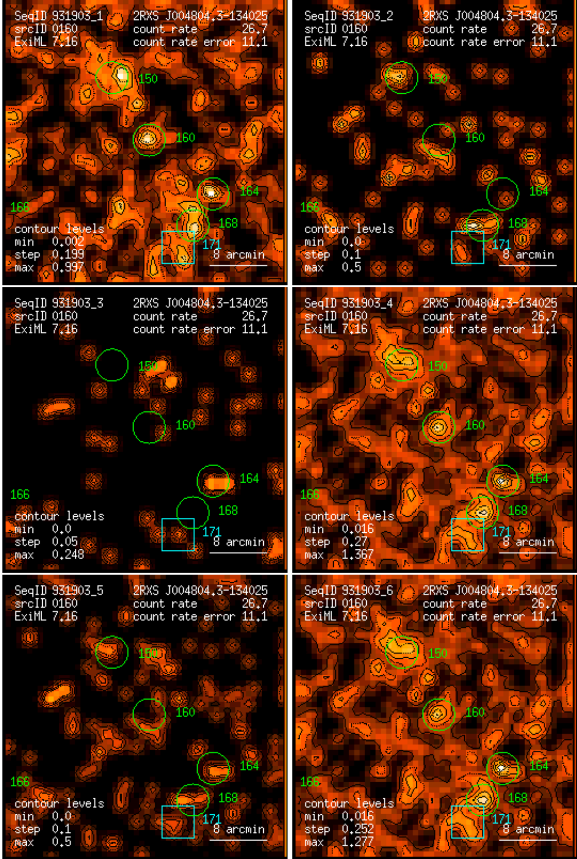
Figure 160: RASS 931903: detection 0160: band rate images, Gaussian filter: (1) PSPC channels 11 – 41, (2) 52 – 90, (3) 91 – 201, (4) 11 – 235, (5) 52 – 201, (6) 11 – 201. Broad band rates in counts/ks. Band rate contour levels in counts/ks/arcmin 2 .
