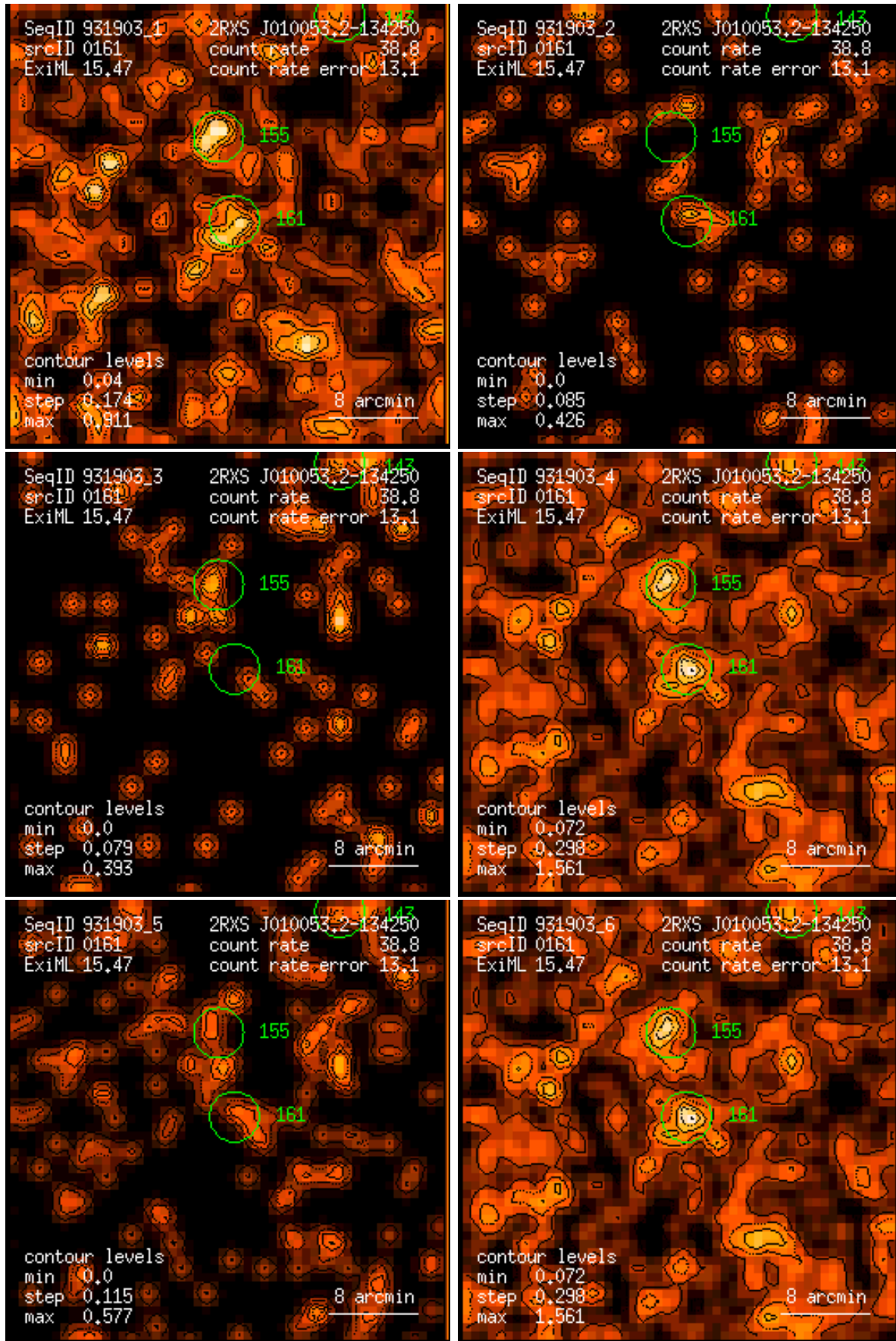
Figure 161: RASS 931903: detection 0161: band rate images, Gaussian filter: (1) PSPC channels 11 – 41, (2) 52 – 90, (3) 91 – 201, (4) 11 – 235, (5) 52 – 201, (6) 11 – 201. Broad band rates in counts/ks. Band rate contour levels in counts/ks/arcmin 2 .
