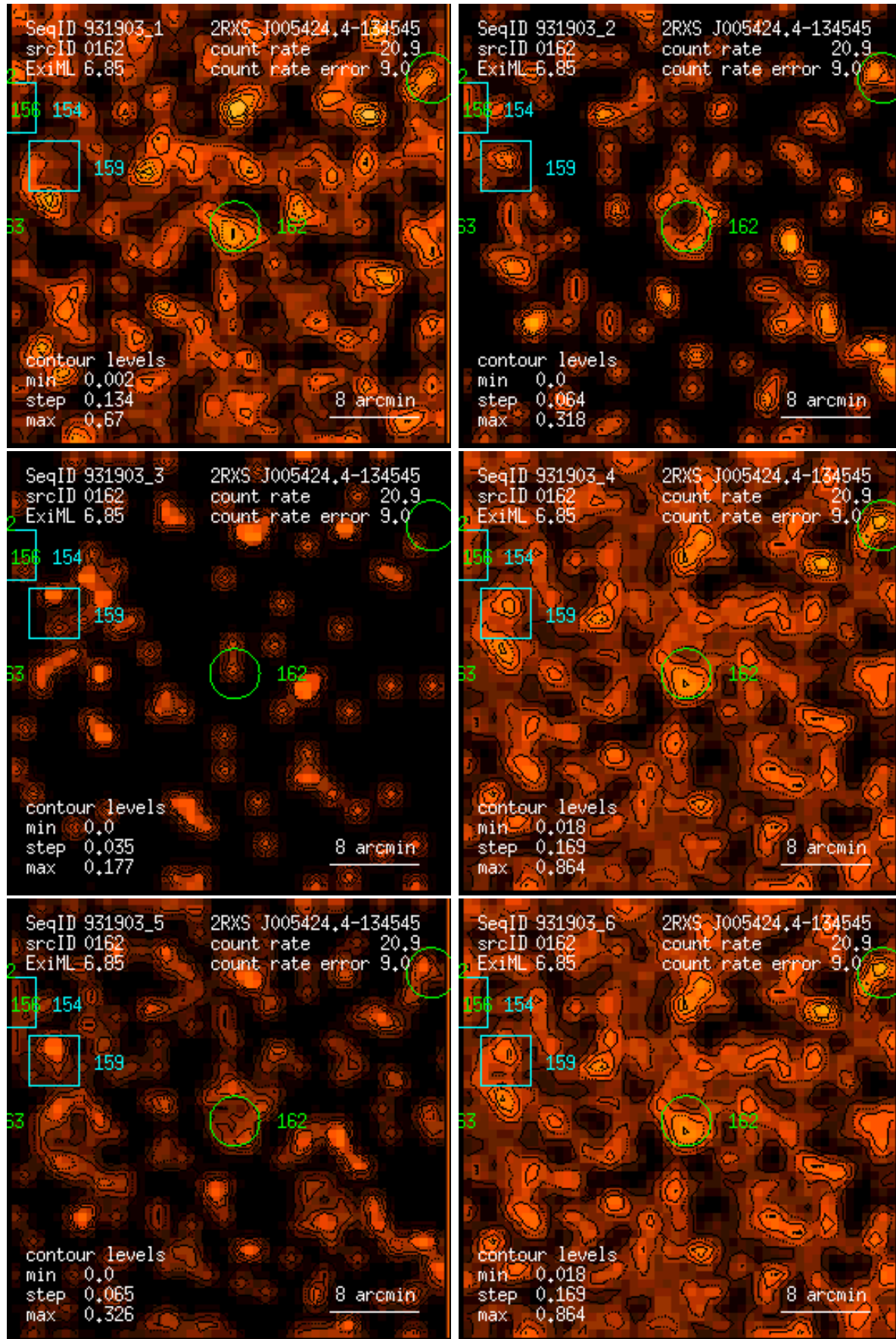
Figure 162: RASS 931903: detection 0162: band rate images, Gaussian filter: (1) PSPC channels 11 – 41, (2) 52 – 90, (3) 91 – 201, (4) 11 – 235, (5) 52 – 201, (6) 11 – 201. Broad band rates in counts/ks. Band rate contour levels in counts/ks/arcmin 2 .
