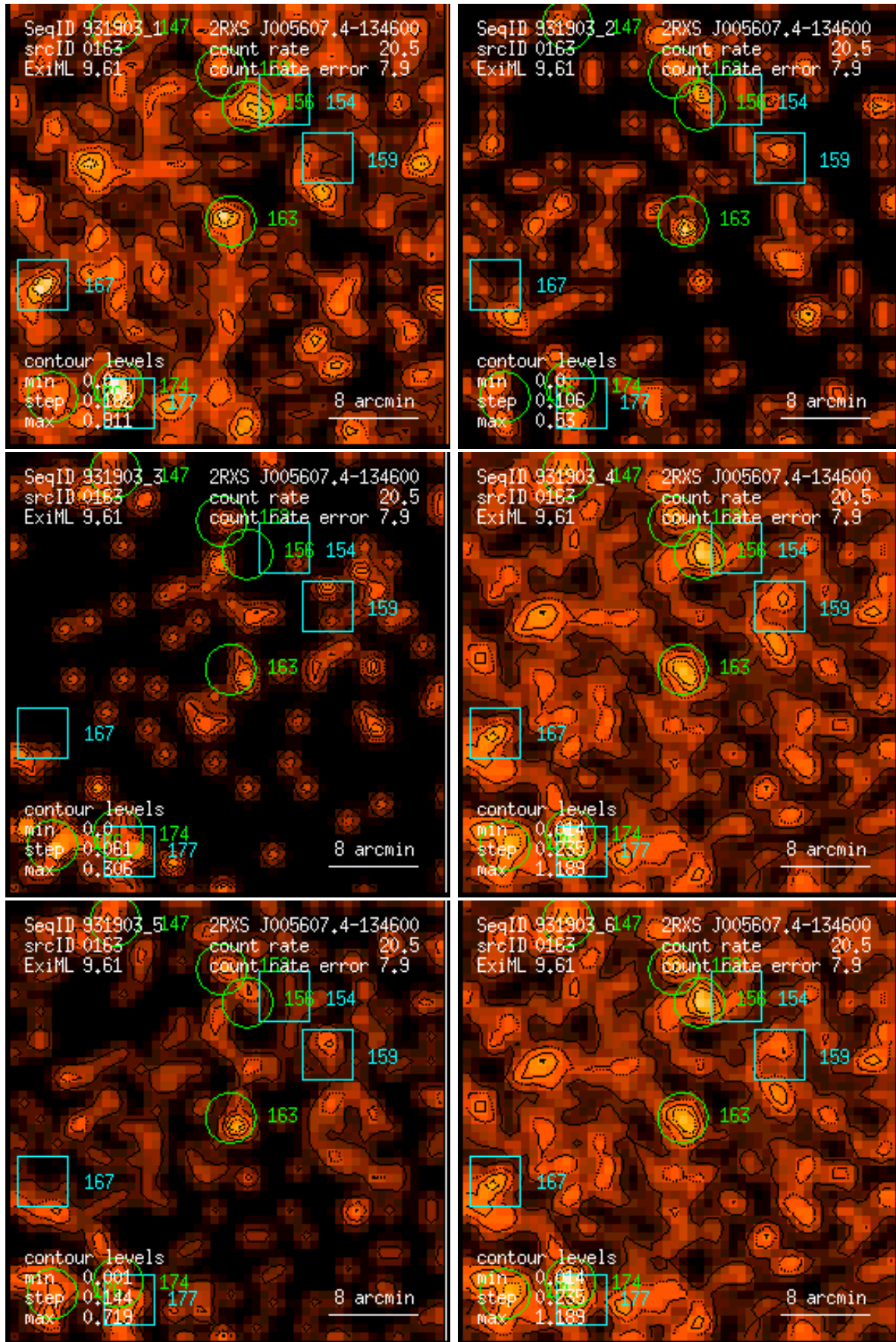
Figure 163: RASS 931903: detection 0163: band rate images, Gaussian filter: (1) PSPC channels 11 – 41, (2) 52 – 90, (3) 91 – 201, (4) 11 – 235, (5) 52 – 201, (6) 11 – 201. Broad band rates in counts/ks. Band rate contour levels in counts/ks/arcmin 2 .
