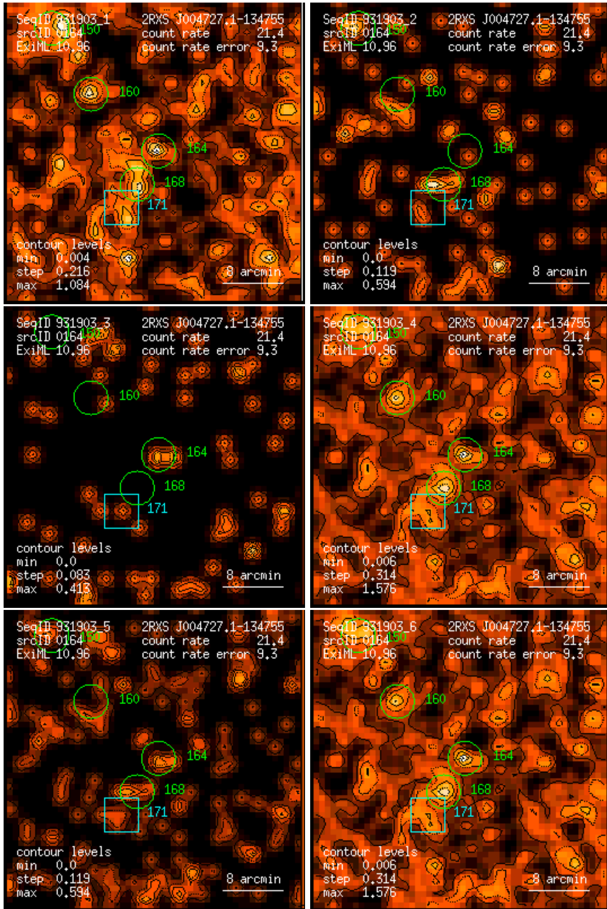
Figure 164: RASS 931903: detection 0164: band rate images, Gaussian filter: (1) PSPC channels 11 – 41, (2) 52 – 90, (3) 91 – 201, (4) 11 – 235, (5) 52 – 201, (6) 11 – 201. Broad band rates in counts/ks. Band rate contour levels in counts/ks/arcmin 2 .
