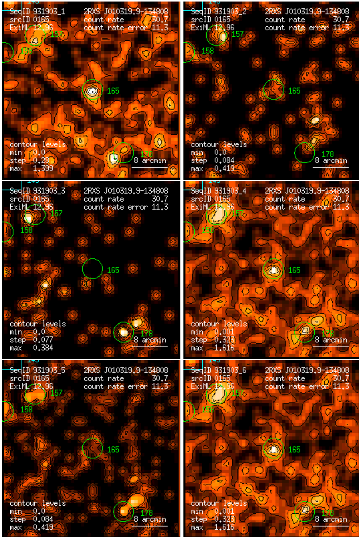
Figure 165: RASS 931903: detection 0165: band rate images, Gaussian filter: (1) PSPC channels 11 – 41, (2) 52 – 90, (3) 91 – 201, (4) 11 – 235, (5) 52 – 201, (6) 11 – 201. Broad band rates in counts/ks. Band rate contour levels in counts/ks/arcmin 2 .
