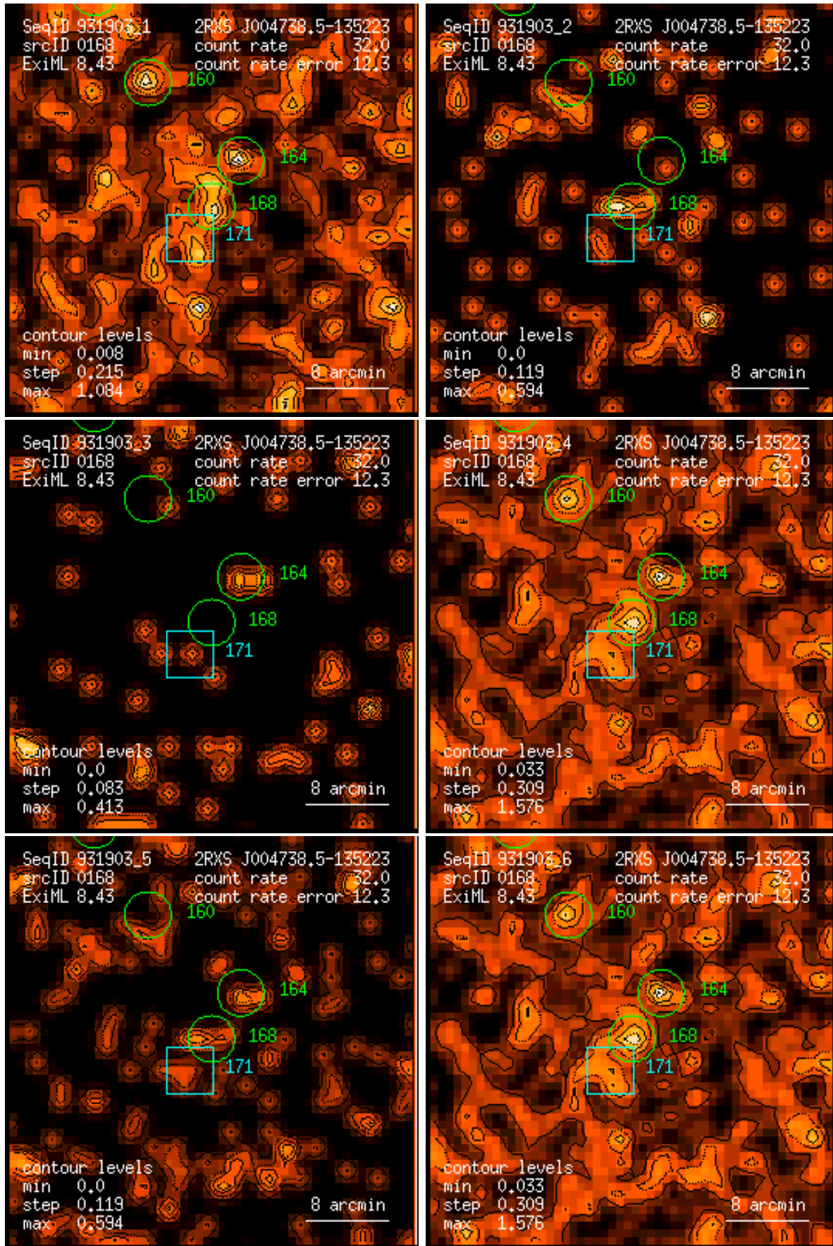
Figure 168: RASS 931903: detection 0168: band rate images, Gaussian filter: (1) PSPC channels 11 – 41, (2) 52 – 90, (3) 91 – 201, (4) 11 – 235, (5) 52 – 201, (6) 11 – 201. Broad band rates in counts/ks. Band rate contour levels in counts/ks/arcmin 2 .
