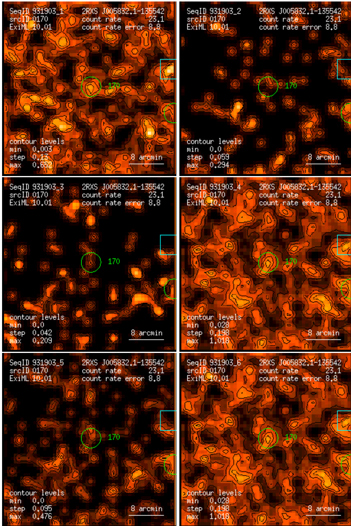
Figure 170: RASS 931903: detection 0170: band rate images, Gaussian filter: (1) PSPC channels 11 – 41, (2) 52 – 90, (3) 91 – 201, (4) 11 – 235, (5) 52 – 201, (6) 11 – 201. Broad band rates in counts/ks. Band rate contour levels in counts/ks/arcmin 2 .
