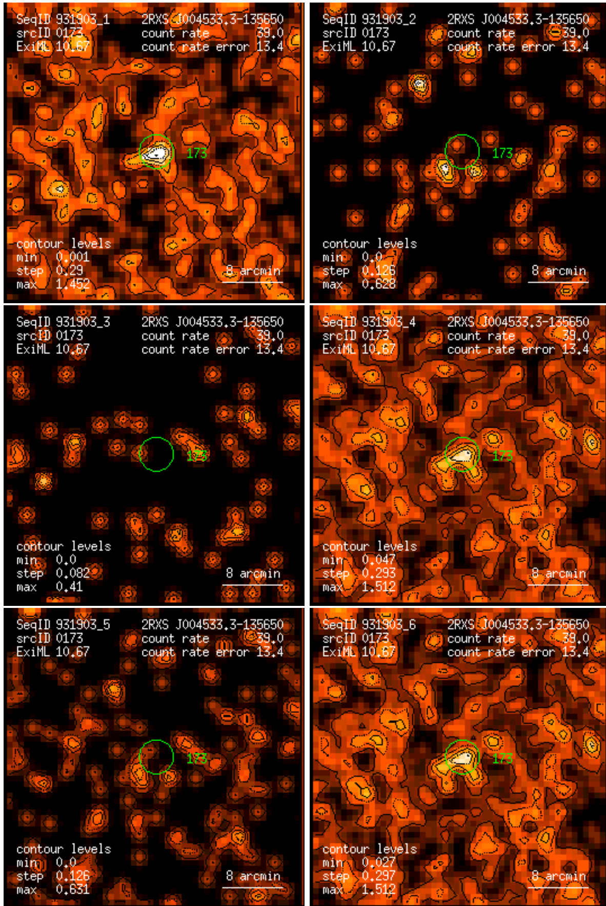
Figure 173: RASS 931903: detection 0173: band rate images, Gaussian filter: (1) PSPC channels 11 – 41, (2) 52 – 90, (3) 91 – 201, (4) 11 – 235, (5) 52 – 201, (6) 11 – 201. Broad band rates in counts/ks. Band rate contour levels in counts/ks/arcmin 2 .
