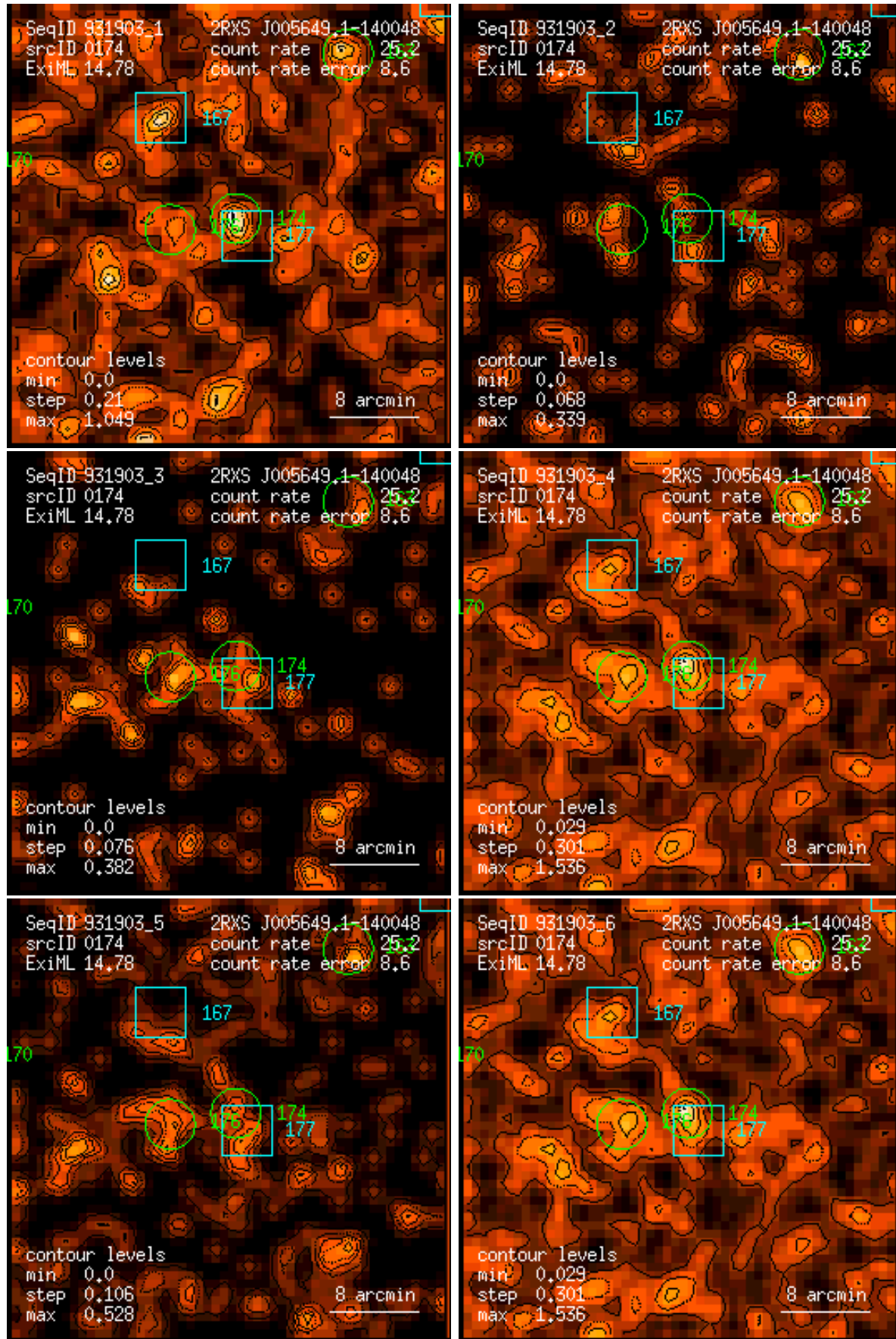
Figure 174: RASS 931903: detection 0174: band rate images, Gaussian filter: (1) PSPC channels 11 – 41, (2) 52 – 90, (3) 91 – 201, (4) 11 – 235, (5) 52 – 201, (6) 11 – 201. Broad band rates in counts/ks. Band rate contour levels in counts/ks/arcmin 2 .
