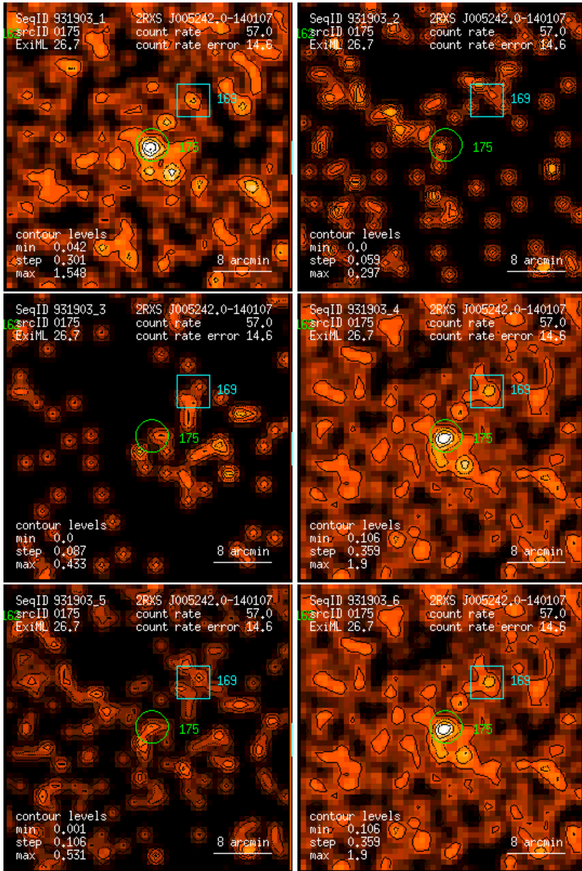
Figure 175: RASS 931903: detection 0175: band rate images, Gaussian filter: (1) PSPC channels 11 – 41, (2) 52 – 90, (3) 91 – 201, (4) 11 – 235, (5) 52 – 201, (6) 11 – 201. Broad band rates in counts/ks. Band rate contour levels in counts/ks/arcmin 2 .
