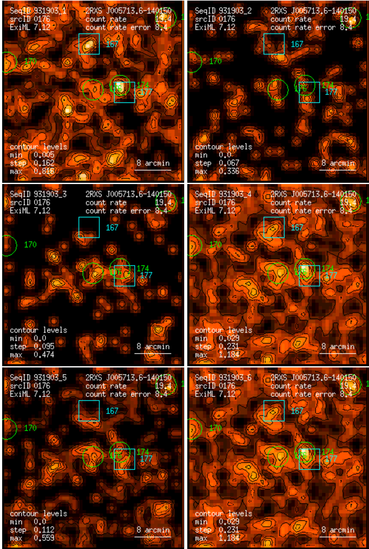
Figure 176: RASS 931903: detection 0176: band rate images, Gaussian filter: (1) PSPC channels 11 – 41, (2) 52 – 90, (3) 91 – 201, (4) 11 – 235, (5) 52 – 201, (6) 11 – 201. Broad band rates in counts/ks. Band rate contour levels in counts/ks/arcmin 2 .
