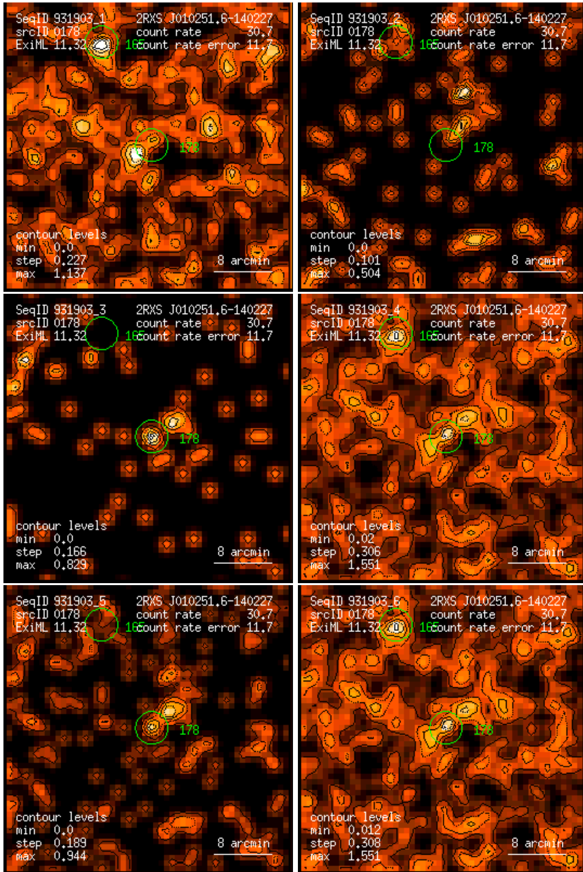
Figure 178: RASS 931903: detection 0178: band rate images, Gaussian filter: (1) PSPC channels 11 – 41, (2) 52 – 90, (3) 91 – 201, (4) 11 – 235, (5) 52 – 201, (6) 11 – 201. Broad band rates in counts/ks. Band rate contour levels in counts/ks/arcmin 2 .
