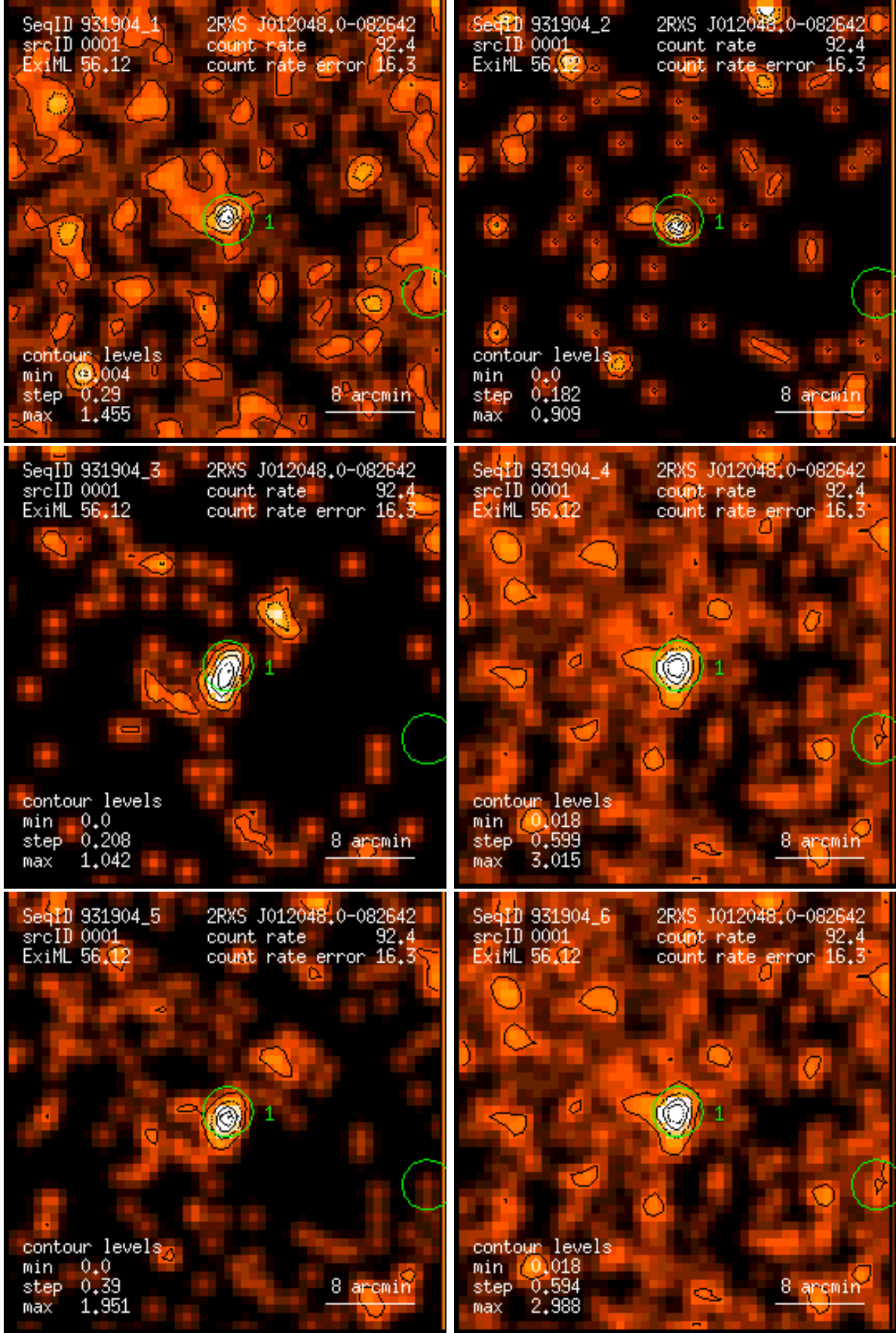
Figure 1: RASS 931904: detection 0001: band rate images, Gaussian filter: (1) PSPC channels 11 – 41, (2) 52 – 90, (3) 91 – 201, (4) 11 – 235, (5) 52 – 201, (6) 11 – 201. Broad band rates in counts/ks. Band rate contour levels in counts/ks/arcmin 2 .
