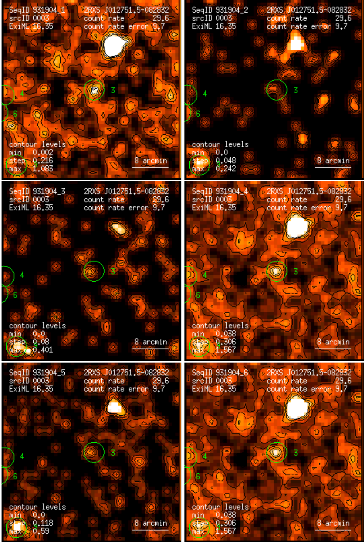
Figure 3: RASS 931904: detection 0003: band rate images, Gaussian filter: (1) PSPC channels 11 – 41, (2) 52 – 90, (3) 91 – 201, (4) 11 – 235, (5) 52 – 201, (6) 11 – 201. Broad band rates in counts/ks. Band rate contour levels in counts/ks/arcmin 2 .
