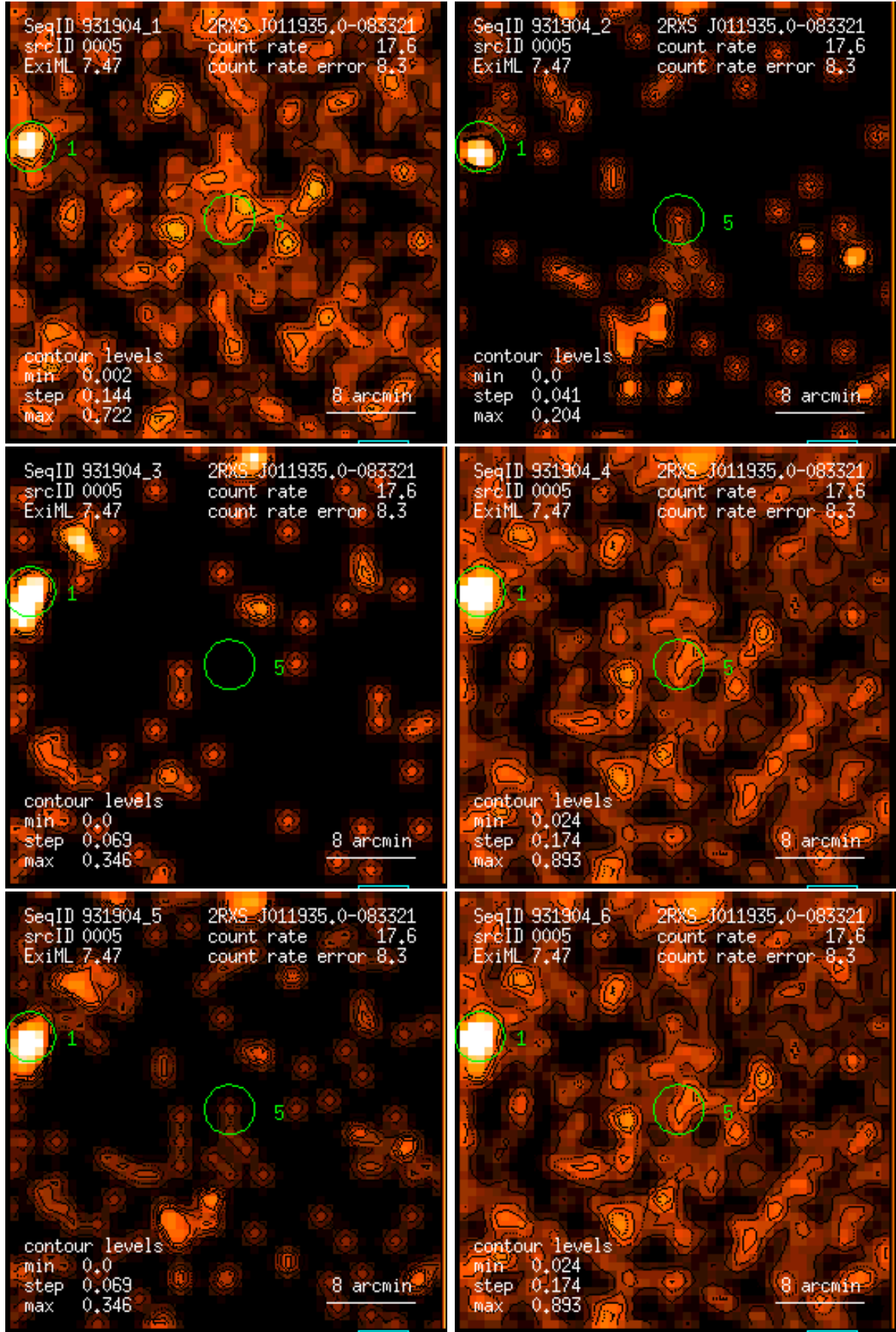
Figure 5: RASS 931904: detection 0005: band rate images, Gaussian filter: (1) PSPC channels 11 – 41, (2) 52 – 90, (3) 91 – 201, (4) 11 – 235, (5) 52 – 201, (6) 11 – 201. Broad band rates in counts/ks. Band rate contour levels in counts/ks/arcmin 2 .
