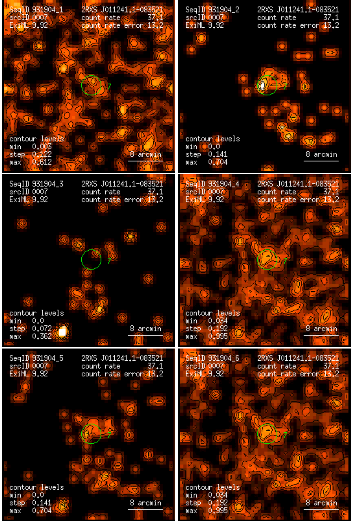
Figure 7: RASS 931904: detection 0007: band rate images, Gaussian filter: (1) PSPC channels 11 – 41, (2) 52 – 90, (3) 91 – 201, (4) 11 – 235, (5) 52 – 201, (6) 11 – 201. Broad band rates in counts/ks. Band rate contour levels in counts/ks/arcmin 2 .
