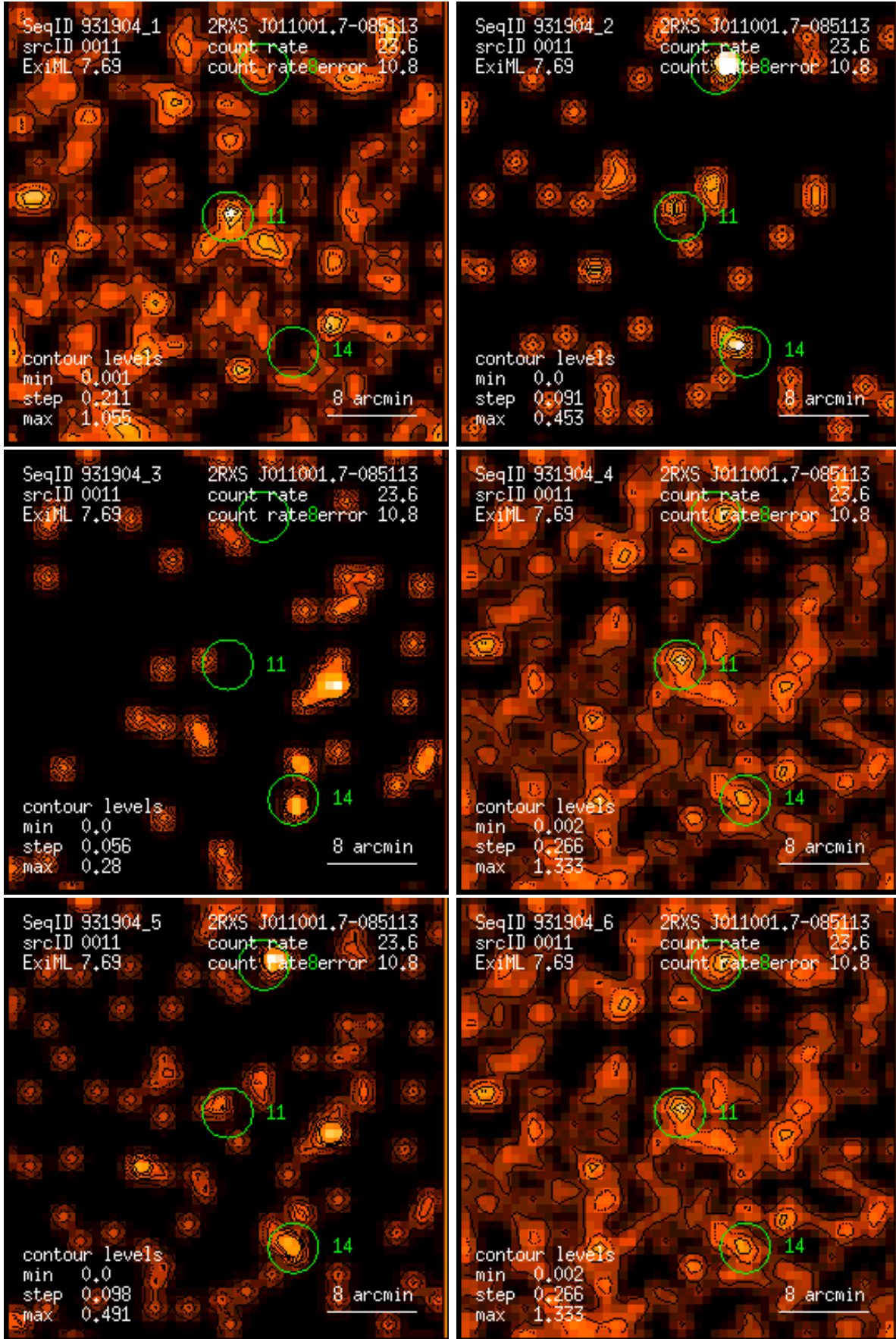
Figure 11: RASS 931904: detection 0011: band rate images, Gaussian filter: (1) PSPC channels 11 – 41, (2) 52 – 90, (3) 91 – 201, (4) 11 – 235, (5) 52 – 201, (6) 11 – 201. Broad band rates in counts/ks. Band rate contour levels in counts/ks/arcmin 2 .
