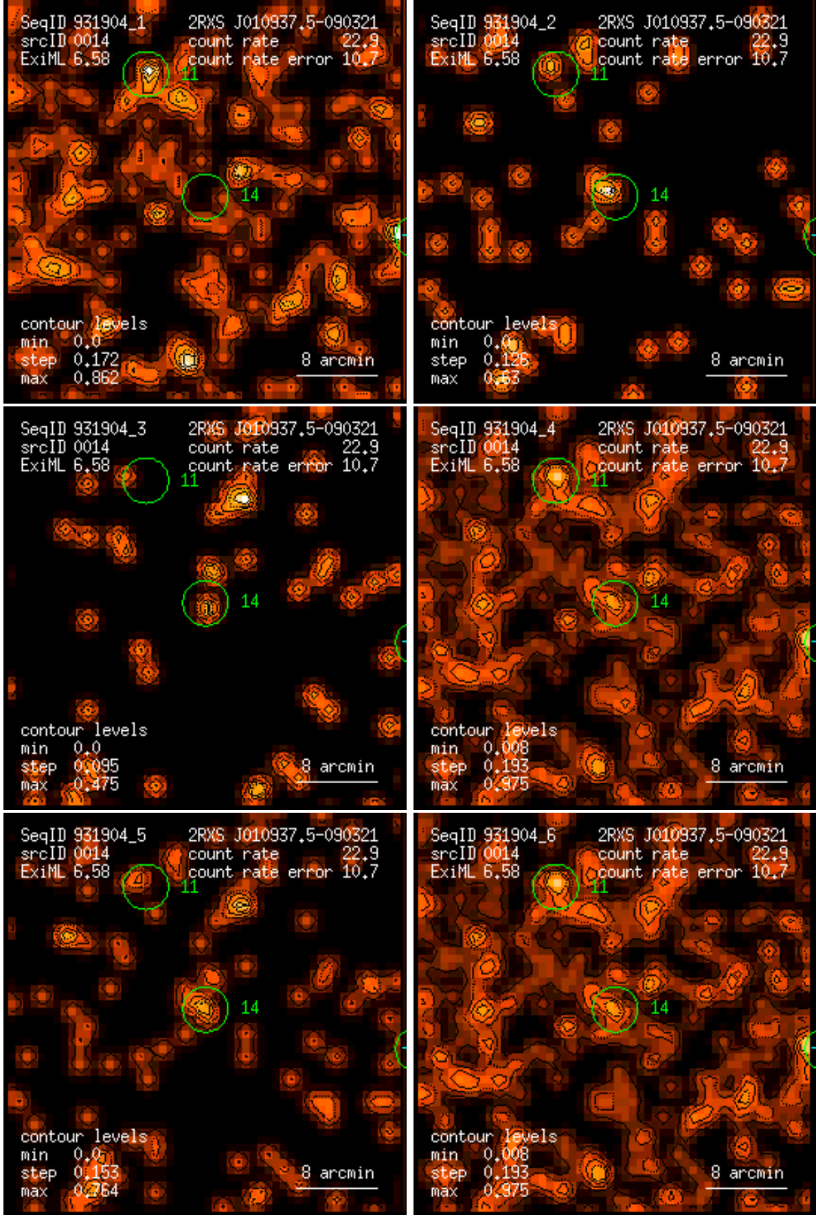
Figure 14: RASS 931904: detection 0014: band rate images, Gaussian filter: (1) PSPC channels 11 – 41, (2) 52 – 90, (3) 91 – 201, (4) 11 – 235, (5) 52 – 201, (6) 11 – 201. Broad band rates in counts/ks. Band rate contour levels in counts/ks/arcmin 2 .
