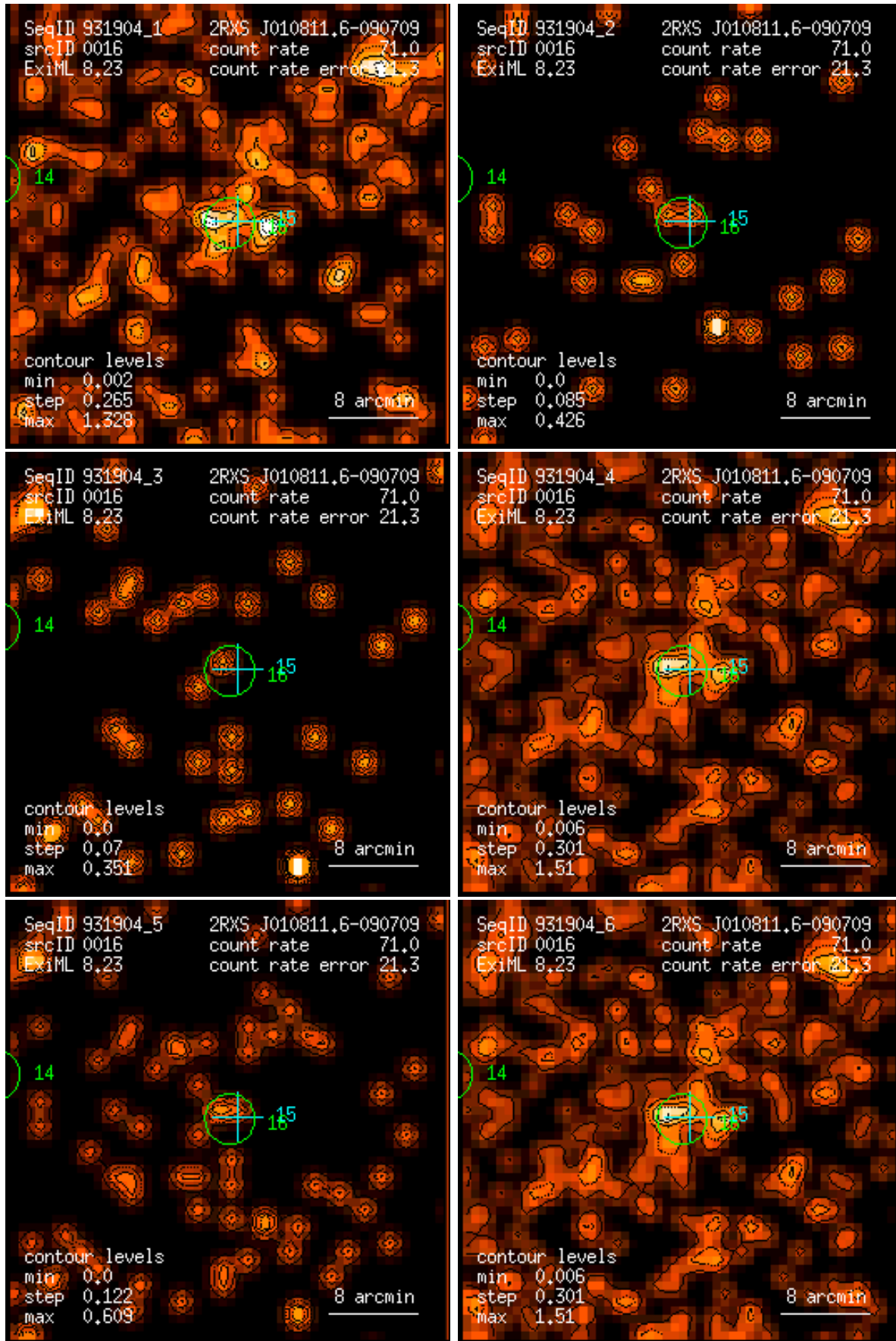
Figure 16: RASS 931904: detection 0016: band rate images, Gaussian filter: (1) PSPC channels 11 – 41, (2) 52 – 90, (3) 91 – 201, (4) 11 – 235, (5) 52 – 201, (6) 11 – 201. Broad band rates in counts/ks. Band rate contour levels in counts/ks/arcmin 2 .
