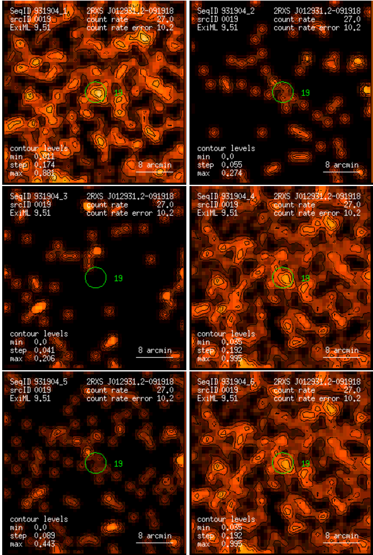
Figure 19: RASS 931904: detection 0019: band rate images, Gaussian filter: (1) PSPC channels 11 – 41, (2) 52 – 90, (3) 91 – 201, (4) 11 – 235, (5) 52 – 201, (6) 11 – 201. Broad band rates in counts/ks. Band rate contour levels in counts/ks/arcmin 2 .
