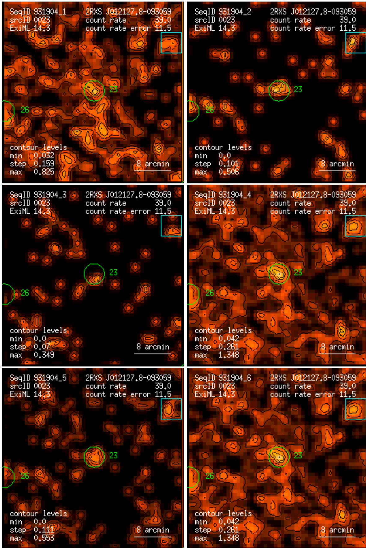
Figure 23: RASS 931904: detection 0023: band rate images, Gaussian filter: (1) PSPC channels 11 – 41, (2) 52 – 90, (3) 91 – 201, (4) 11 – 235, (5) 52 – 201, (6) 11 – 201. Broad band rates in counts/ks. Band rate contour levels in counts/ks/arcmin 2 .
