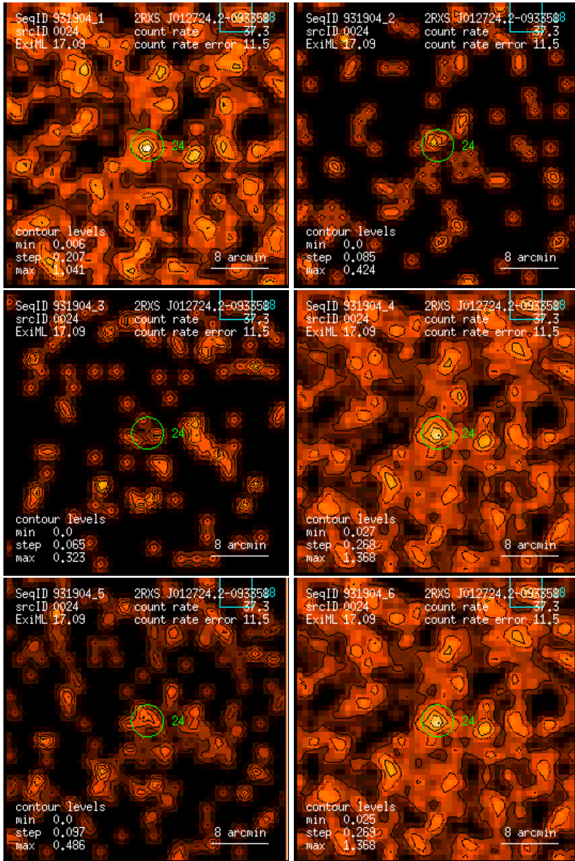
Figure 24: RASS 931904: detection 0024: band rate images, Gaussian filter: (1) PSPC channels 11 – 41, (2) 52 – 90, (3) 91 – 201, (4) 11 – 235, (5) 52 – 201, (6) 11 – 201. Broad band rates in counts/ks. Band rate contour levels in counts/ks/arcmin 2 .
