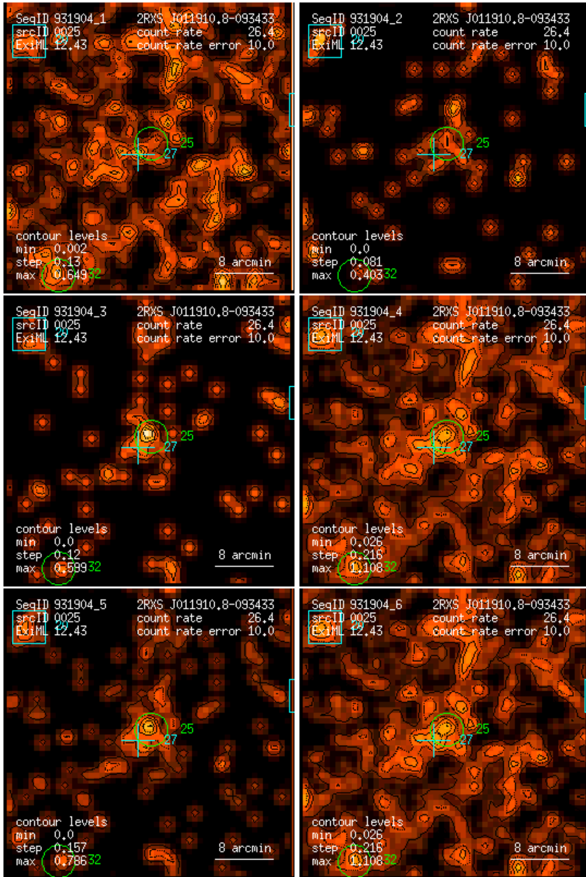
Figure 25: RASS 931904: detection 0025: band rate images, Gaussian filter: (1) PSPC channels 11 – 41, (2) 52 – 90, (3) 91 – 201, (4) 11 – 235, (5) 52 – 201, (6) 11 – 201. Broad band rates in counts/ks. Band rate contour levels in counts/ks/arcmin 2 .
