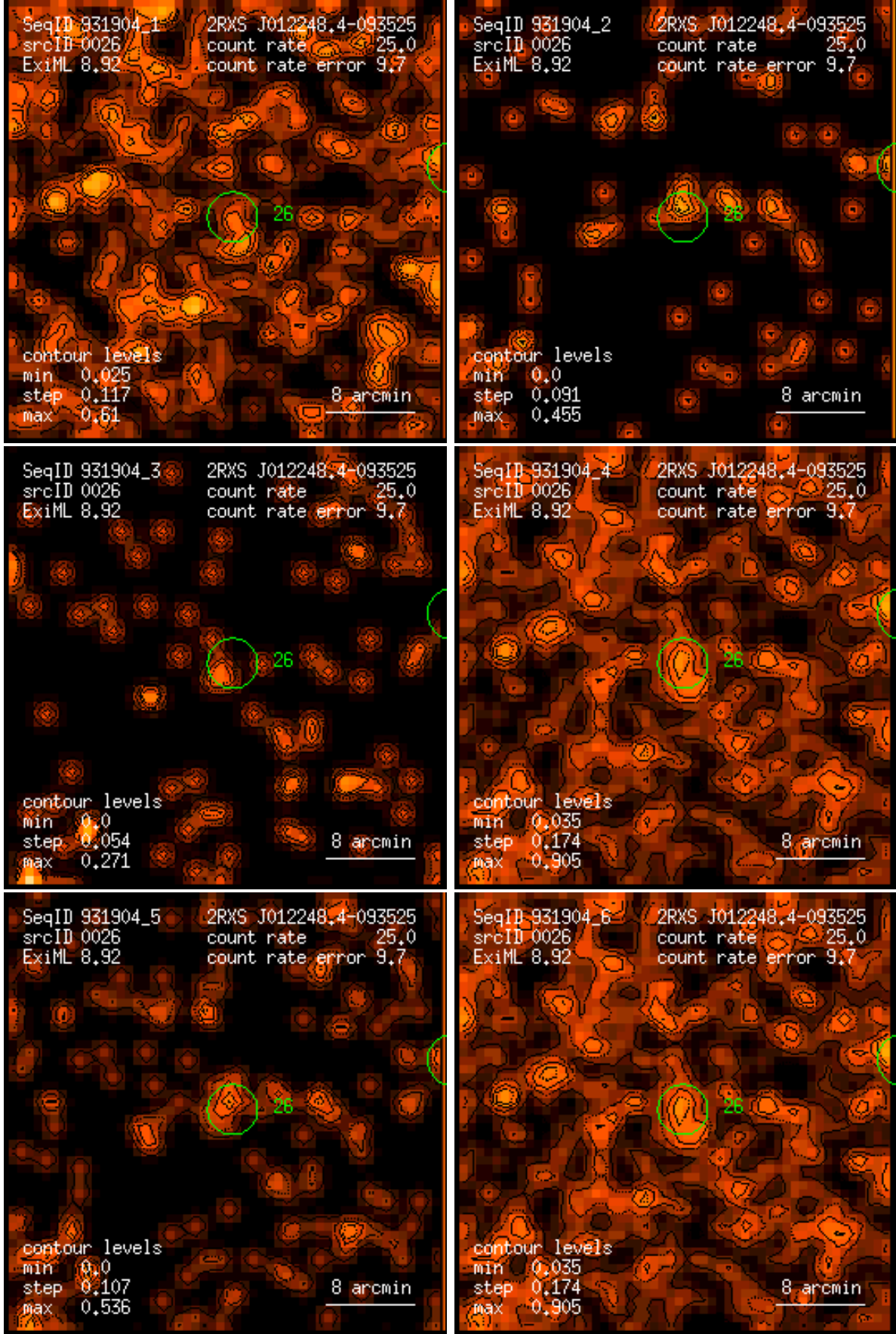
Figure 26: RASS 931904: detection 0026: band rate images, Gaussian filter: (1) PSPC channels 11 – 41, (2) 52 – 90, (3) 91 – 201, (4) 11 – 235, (5) 52 – 201, (6) 11 – 201. Broad band rates in counts/ks. Band rate contour levels in counts/ks/arcmin 2 .
