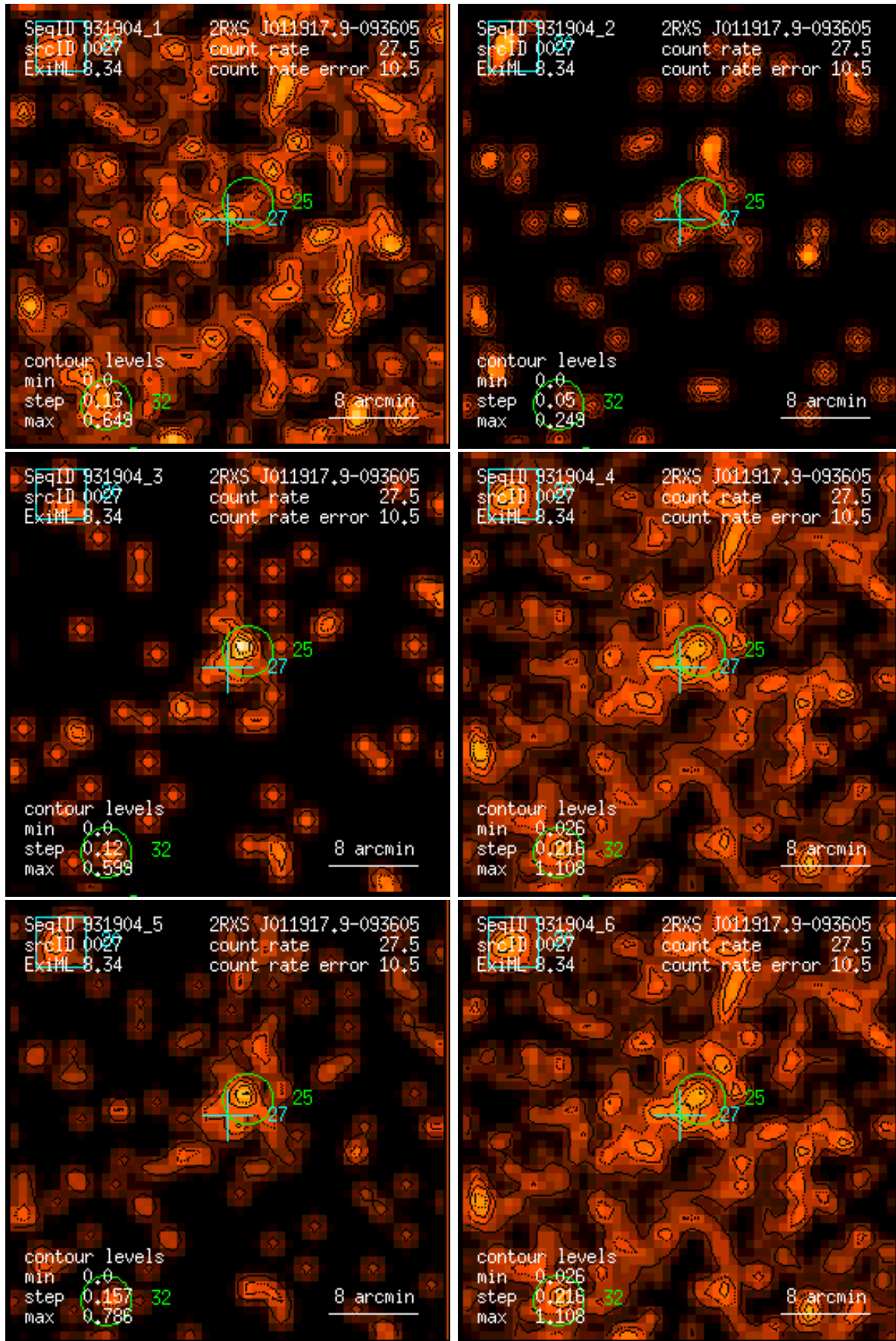
Figure 27: RASS 931904: detection 0027: band rate images, Gaussian filter: (1) PSPC channels 11 – 41, (2) 52 – 90, (3) 91 – 201, (4) 11 – 235, (5) 52 – 201, (6) 11 – 201. Broad band rates in counts/ks. Band rate contour levels in counts/ks/arcmin 2 .
