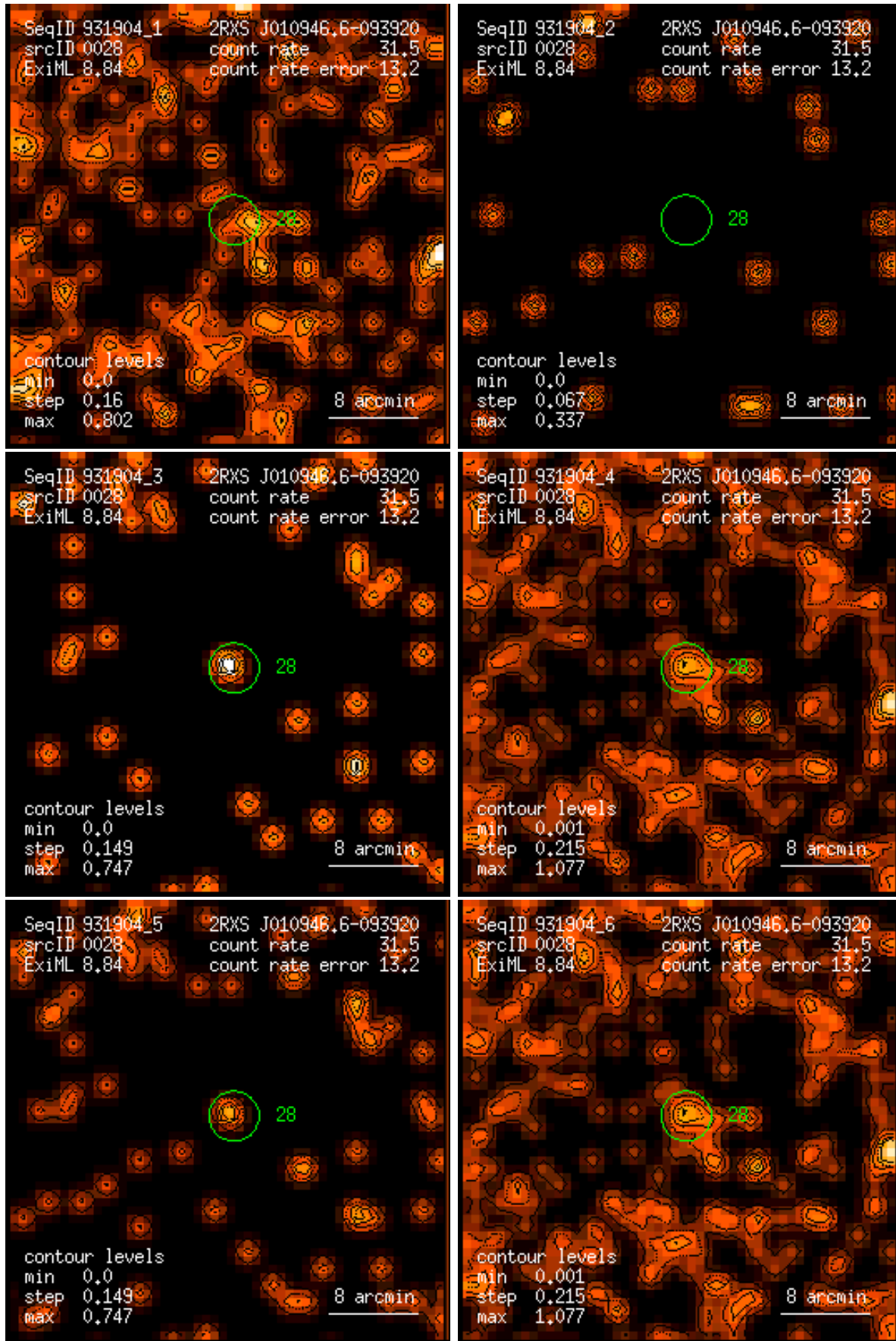
Figure 28: RASS 931904: detection 0028: band rate images, Gaussian filter: (1) PSPC channels 11 – 41, (2) 52 – 90, (3) 91 – 201, (4) 11 – 235, (5) 52 – 201, (6) 11 – 201. Broad band rates in counts/ks. Band rate contour levels in counts/ks/arcmin 2 .
