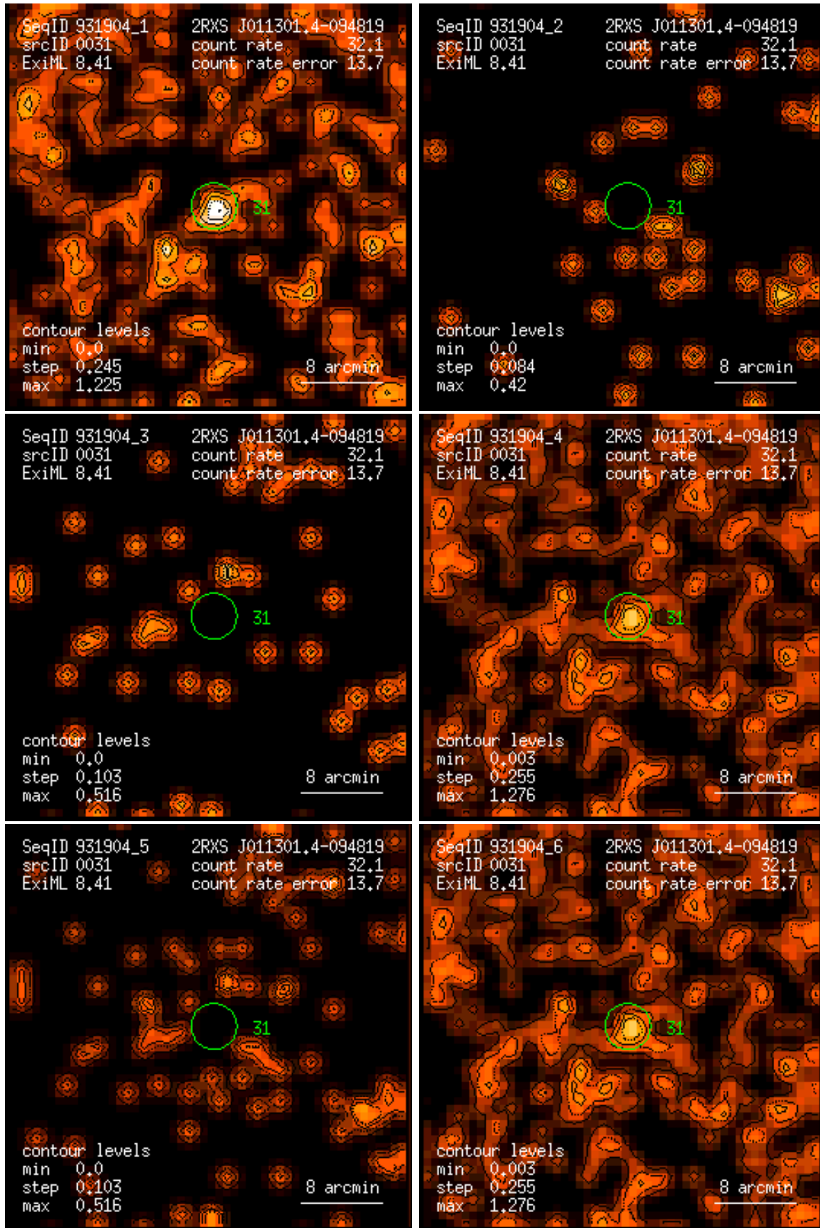
Figure 31: RASS 931904: detection 0031: band rate images, Gaussian filter: (1) PSPC channels 11 – 41, (2) 52 – 90, (3) 91 – 201, (4) 11 – 235, (5) 52 – 201, (6) 11 – 201. Broad band rates in counts/ks. Band rate contour levels in counts/ks/arcmin 2 .
