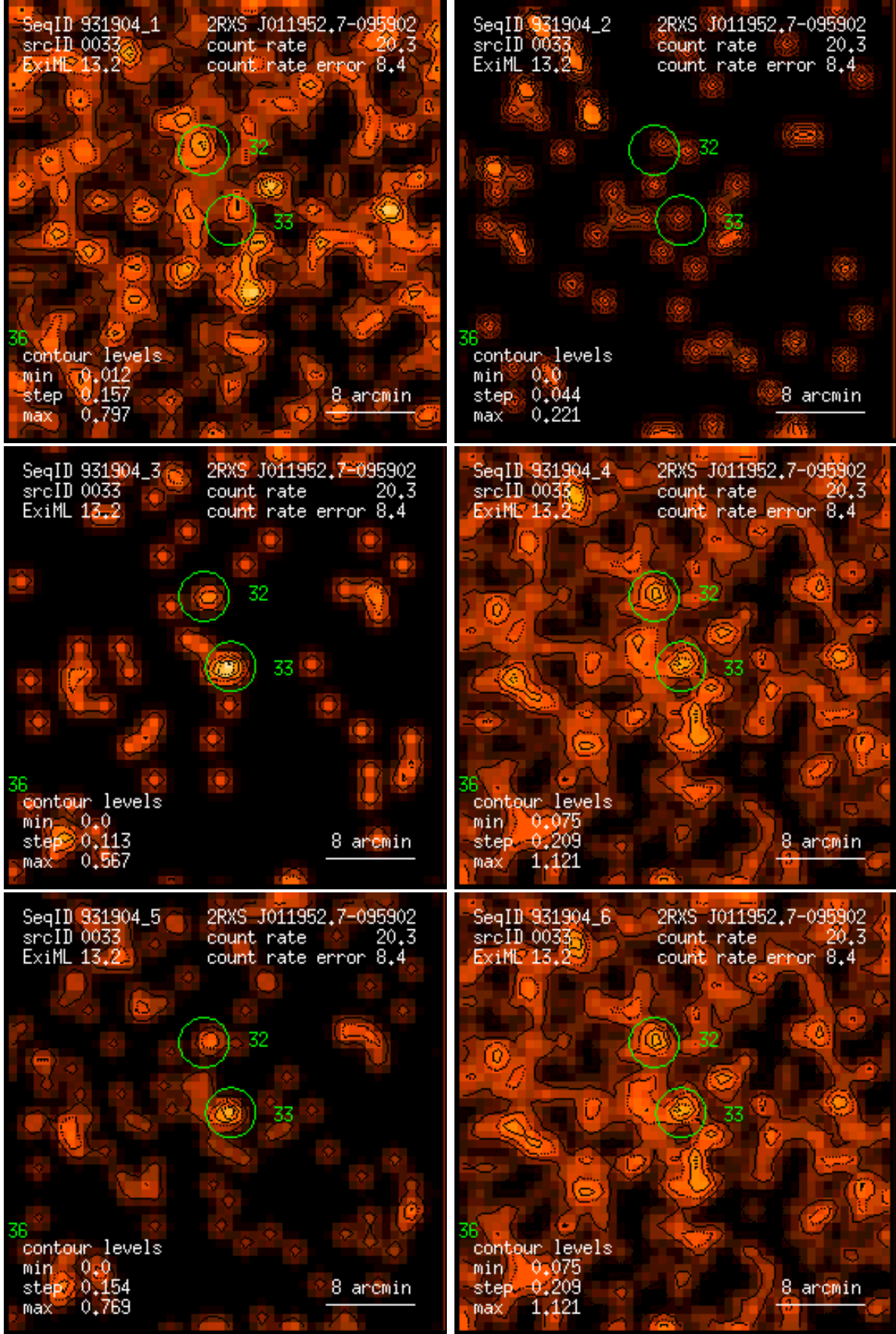
Figure 33: RASS 931904: detection 0033: band rate images, Gaussian filter: (1) PSPC channels 11 – 41, (2) 52 – 90, (3) 91 – 201, (4) 11 – 235, (5) 52 – 201, (6) 11 – 201. Broad band rates in counts/ks. Band rate contour levels in counts/ks/arcmin 2 .
