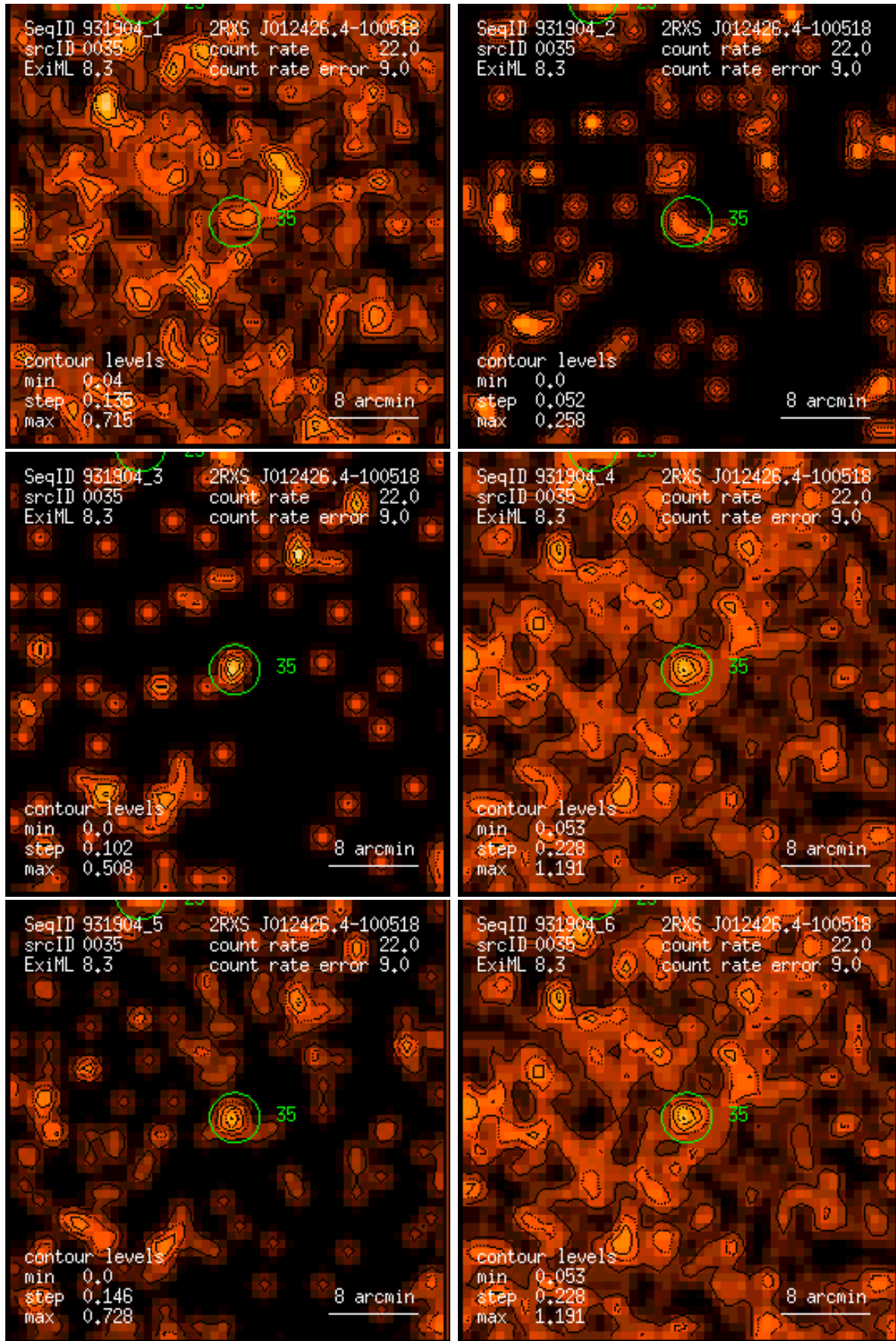
Figure 35: RASS 931904: detection 0035: band rate images, Gaussian filter: (1) PSPC channels 11 – 41, (2) 52 – 90, (3) 91 – 201, (4) 11 – 235, (5) 52 – 201, (6) 11 – 201. Broad band rates in counts/ks. Band rate contour levels in counts/ks/arcmin 2 .
