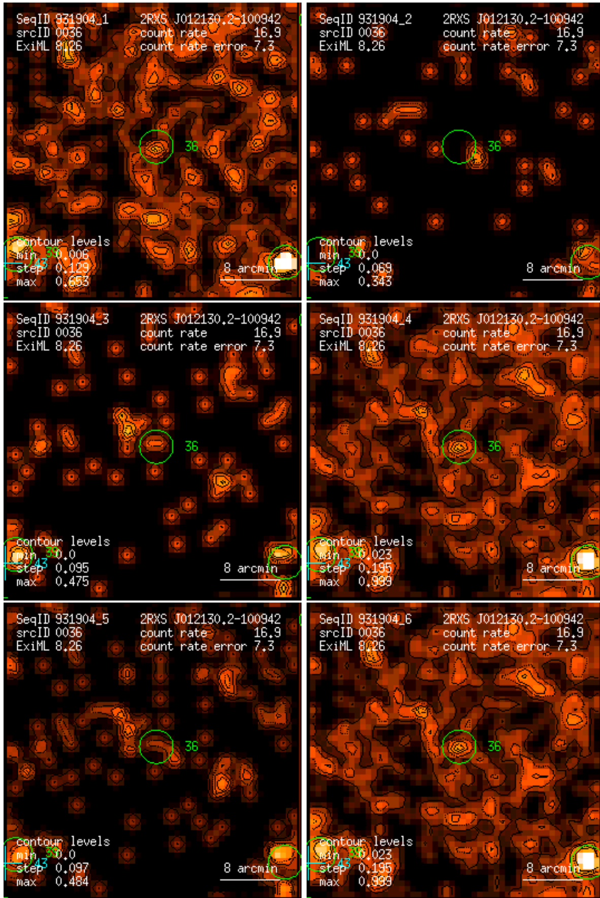
Figure 36: RASS 931904: detection 0036: band rate images, Gaussian filter: (1) PSPC channels 11 – 41, (2) 52 – 90, (3) 91 – 201, (4) 11 – 235, (5) 52 – 201, (6) 11 – 201. Broad band rates in counts/ks. Band rate contour levels in counts/ks/arcmin 2 .
