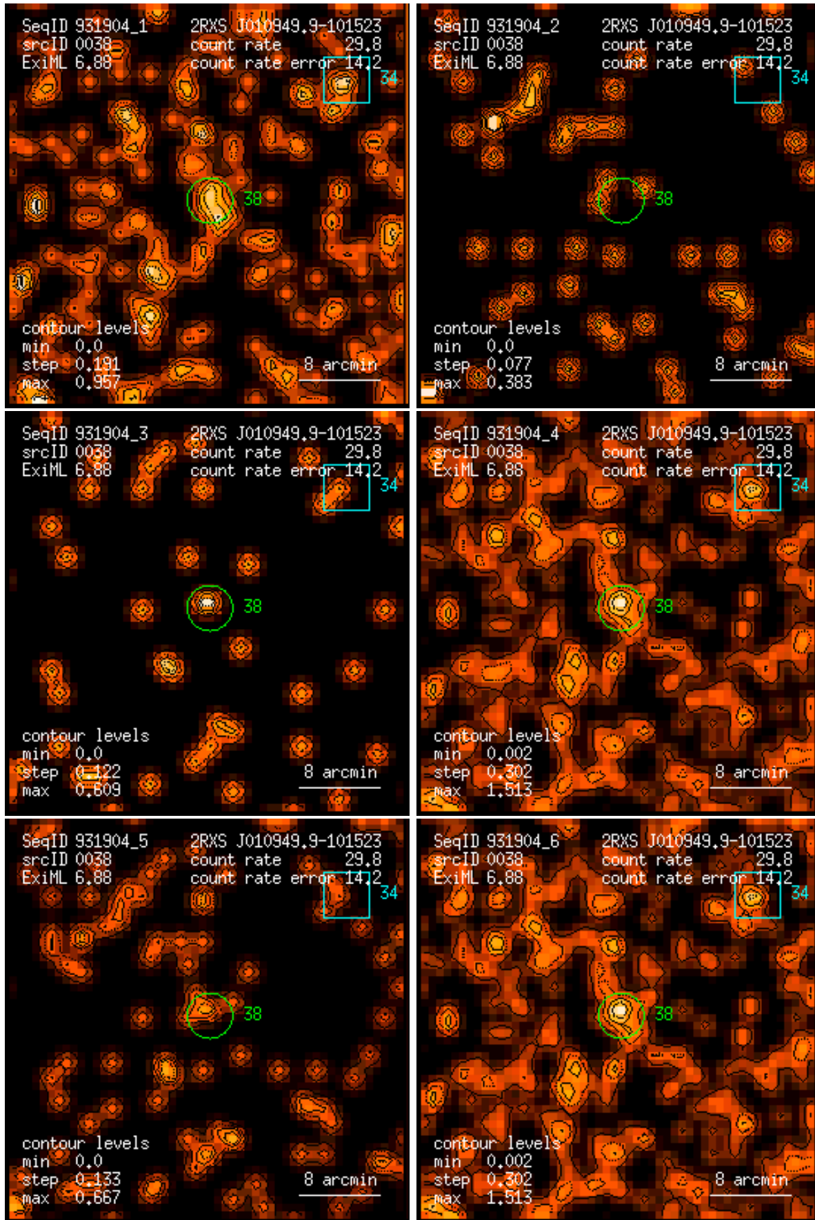
Figure 38: RASS 931904: detection 0038: band rate images, Gaussian filter: (1) PSPC channels 11 – 41, (2) 52 – 90, (3) 91 – 201, (4) 11 – 235, (5) 52 – 201, (6) 11 – 201. Broad band rates in counts/ks. Band rate contour levels in counts/ks/arcmin 2 .
