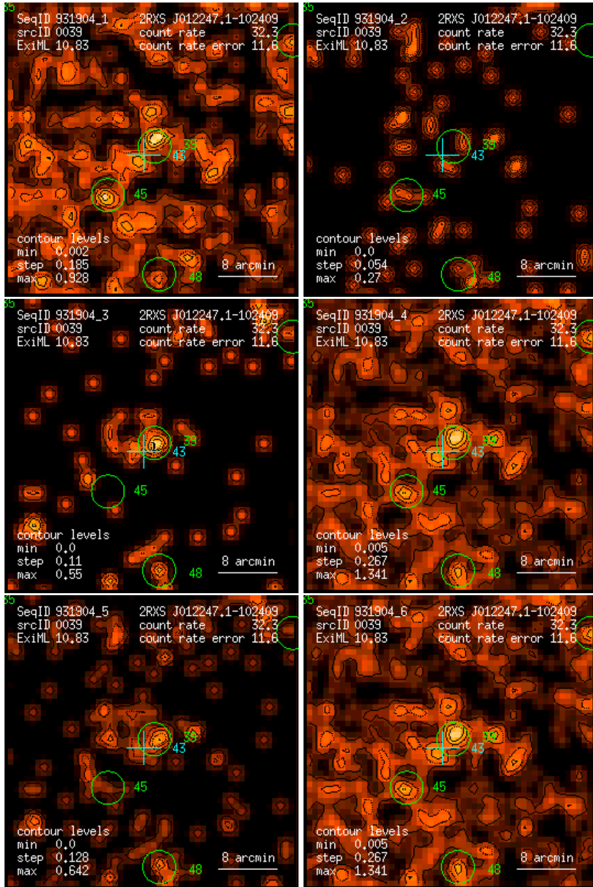
Figure 39: RASS 931904: detection 0039: band rate images, Gaussian filter: (1) PSPC channels 11 – 41, (2) 52 – 90, (3) 91 – 201, (4) 11 – 235, (5) 52 – 201, (6) 11 – 201. Broad band rates in counts/ks. Band rate contour levels in counts/ks/arcmin 2 .
