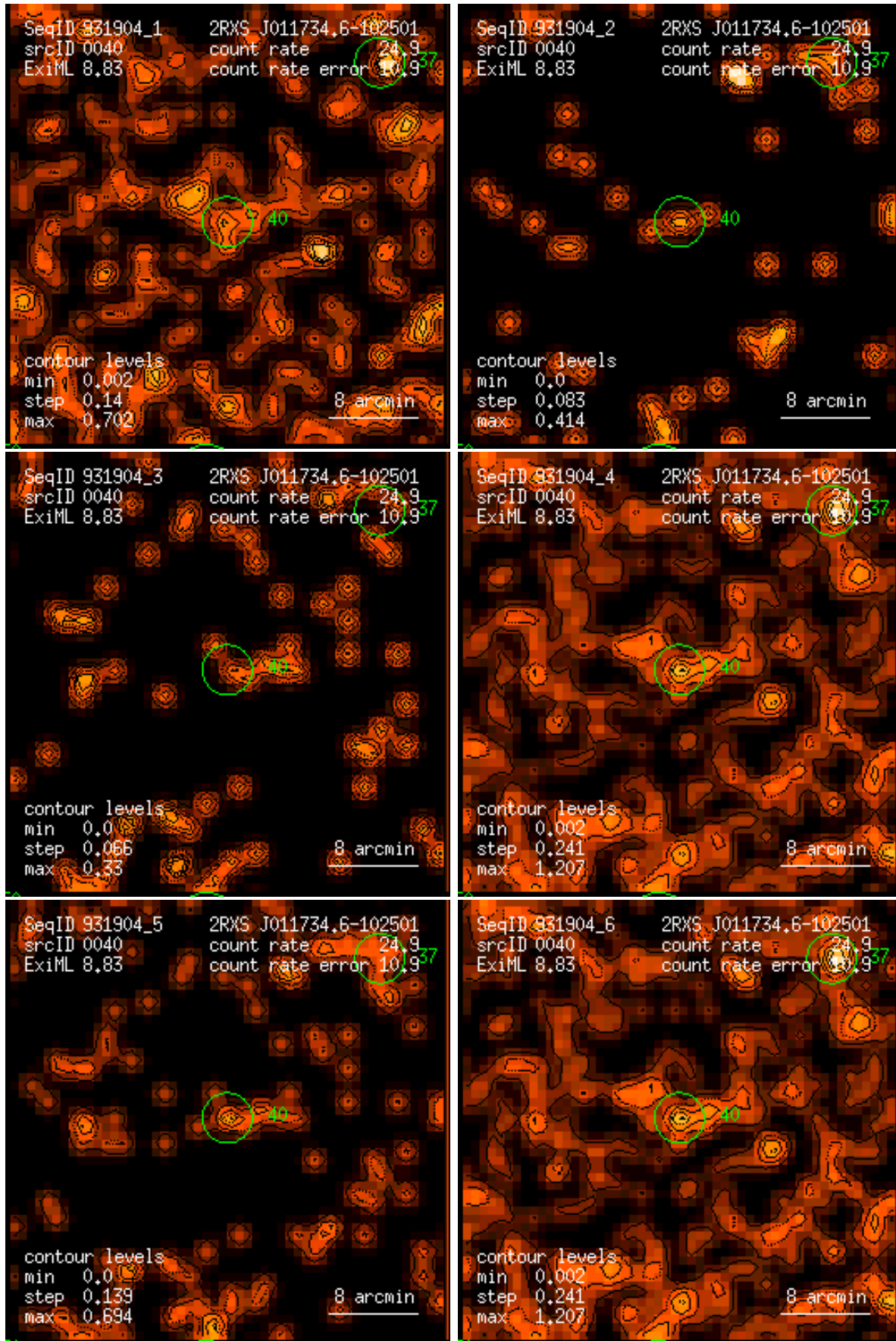
Figure 40: RASS 931904: detection 0040: band rate images, Gaussian filter: (1) PSPC channels 11 – 41, (2) 52 – 90, (3) 91 – 201, (4) 11 – 235, (5) 52 – 201, (6) 11 – 201. Broad band rates in counts/ks. Band rate contour levels in counts/ks/arcmin 2 .
