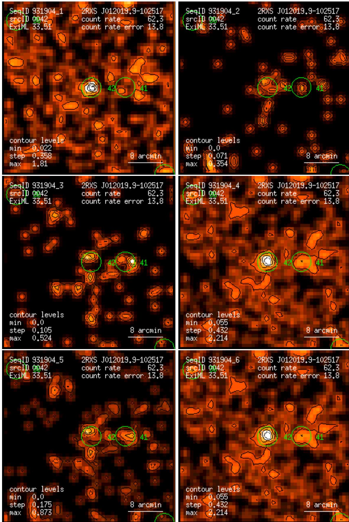
Figure 42: RASS 931904: detection 0042: band rate images, Gaussian filter: (1) PSPC channels 11 – 41, (2) 52 – 90, (3) 91 – 201, (4) 11 – 235, (5) 52 – 201, (6) 11 – 201. Broad band rates in counts/ks. Band rate contour levels in counts/ks/arcmin 2 .
